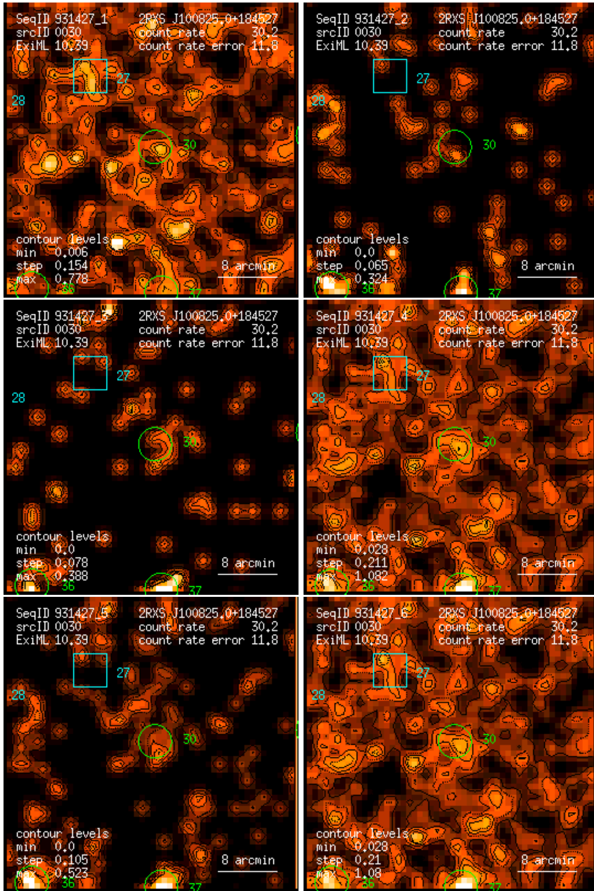
Figure 30: RASS 931427: detection 0030: band rate images, Gaussian filter: (1) PSPC channels 11 – 41, (2) 52 – 90, (3) 91 – 201, (4) 11 – 235, (5) 52 – 201, (6) 11 – 201. Broad band rates in counts/ks. Band rate contour levels in counts/ks/arcmin 2 .
