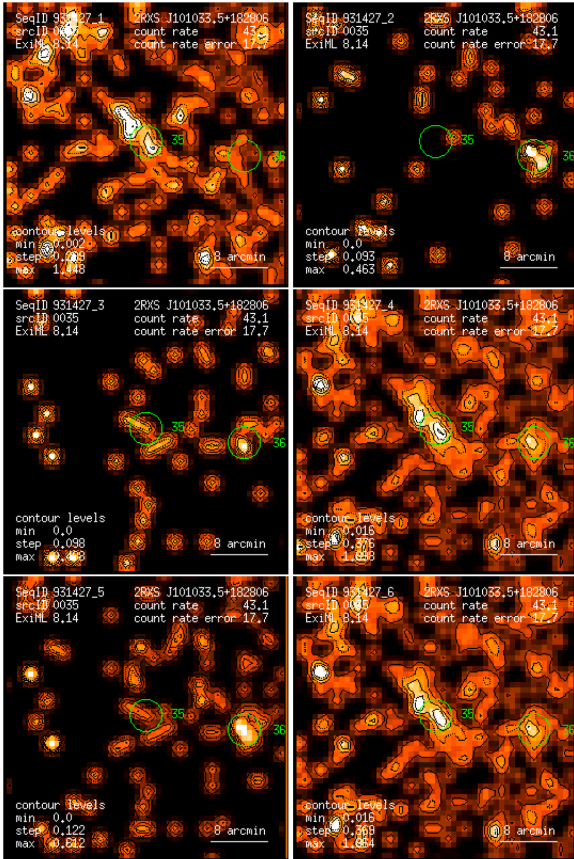
Figure 35: RASS 931427: detection 0035: band rate images, Gaussian filter: (1) PSPC channels 11 – 41, (2) 52 – 90, (3) 91 – 201, (4) 11 – 235, (5) 52 – 201, (6) 11 – 201. Broad band rates in counts/ks. Band rate contour levels in counts/ks/arcmin 2 .
