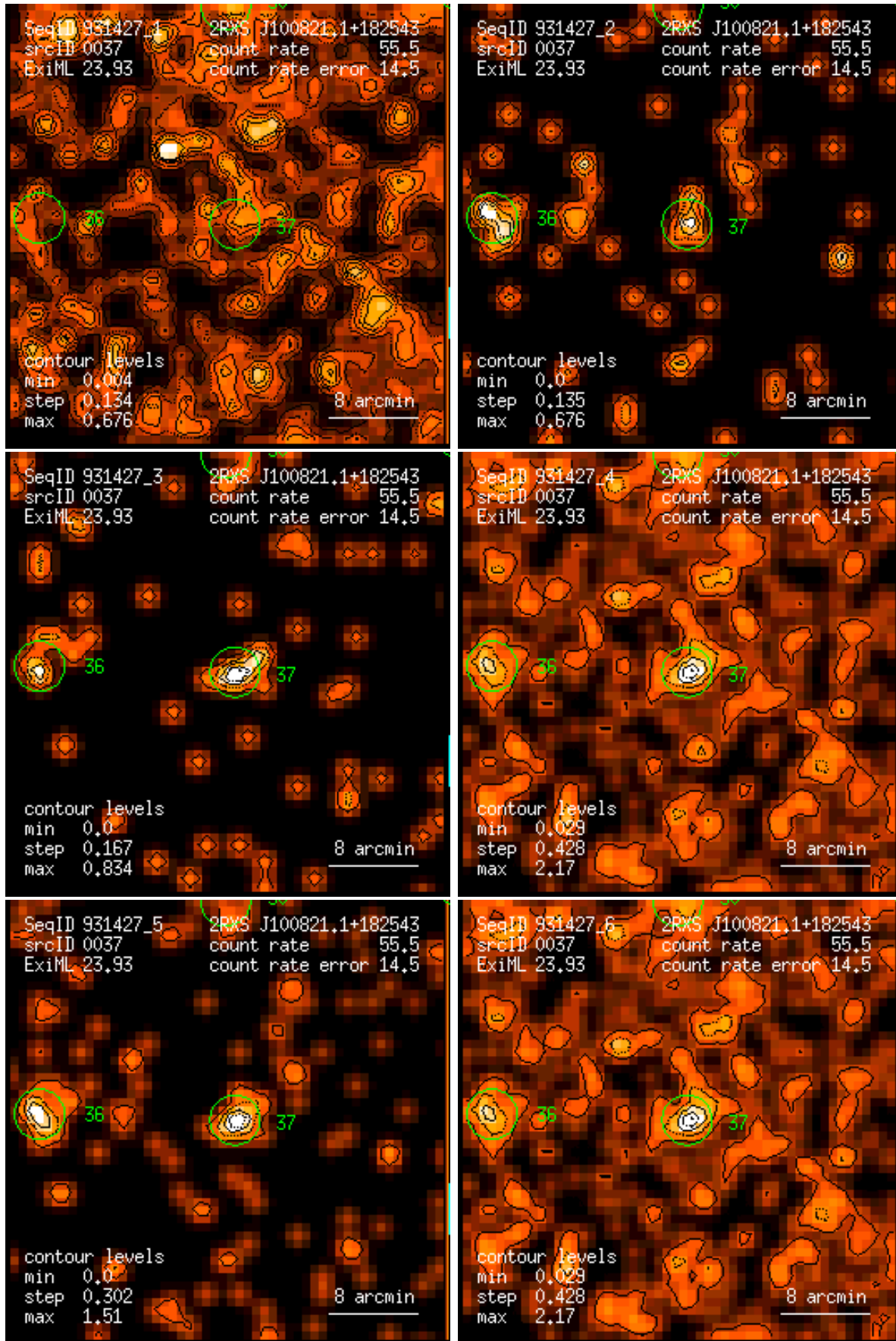
Figure 37: RASS 931427: detection 0037: band rate images, Gaussian filter: (1) PSPC channels 11 – 41, (2) 52 – 90, (3) 91 – 201, (4) 11 – 235, (5) 52 – 201, (6) 11 – 201. Broad band rates in counts/ks. Band rate contour levels in counts/ks/arcmin 2 .
