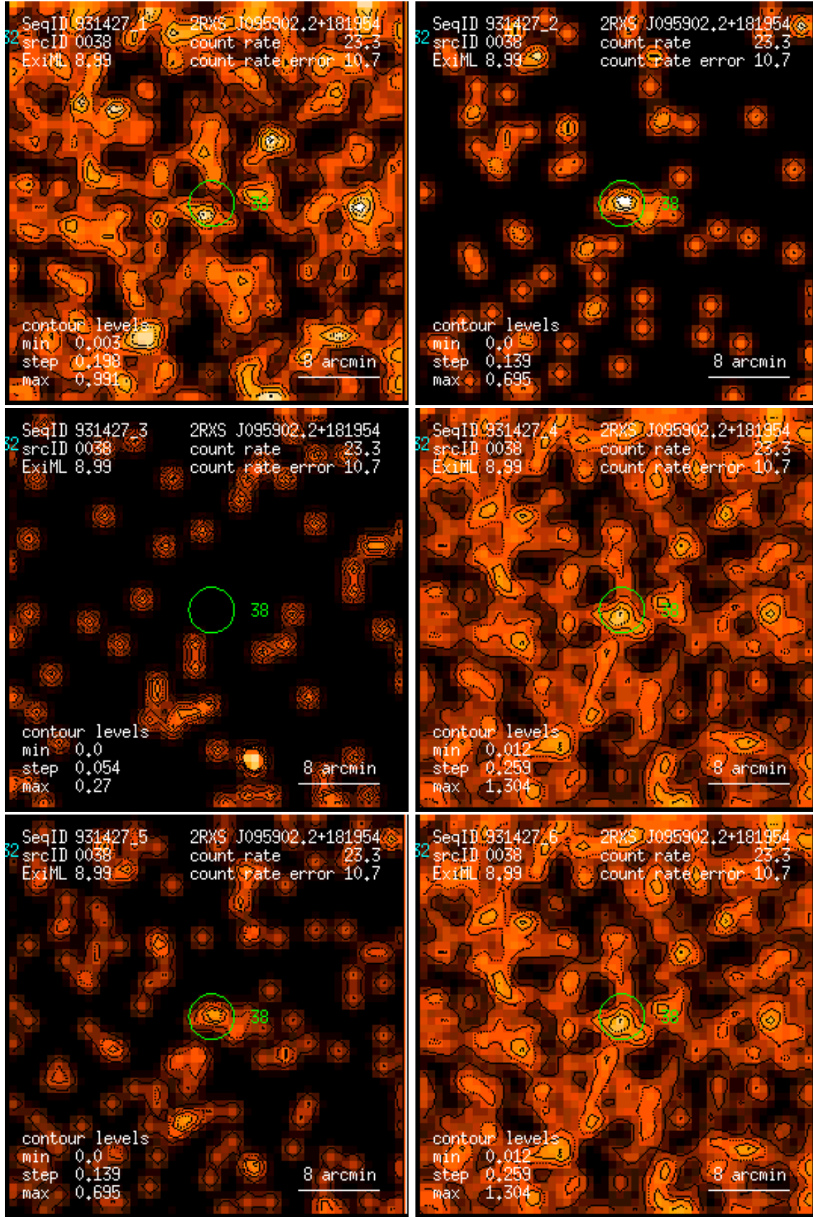
Figure 38: RASS 931427: detection 0038: band rate images, Gaussian filter: (1) PSPC channels 11 – 41, (2) 52 – 90, (3) 91 – 201, (4) 11 – 235, (5) 52 – 201, (6) 11 – 201. Broad band rates in counts/ks. Band rate contour levels in counts/ks/arcmin 2 .
