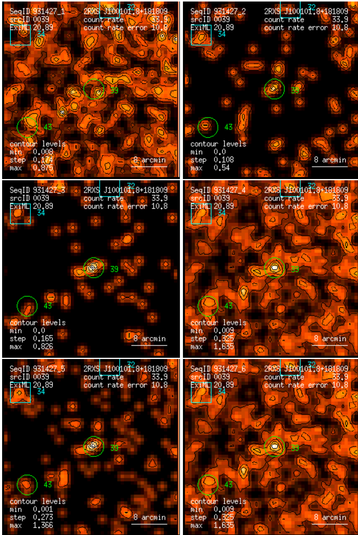
Figure 39: RASS 931427: detection 0039: band rate images, Gaussian filter: (1) PSPC channels 11 – 41, (2) 52 – 90, (3) 91 – 201, (4) 11 – 235, (5) 52 – 201, (6) 11 – 201. Broad band rates in counts/ks. Band rate contour levels in counts/ks/arcmin 2 .
