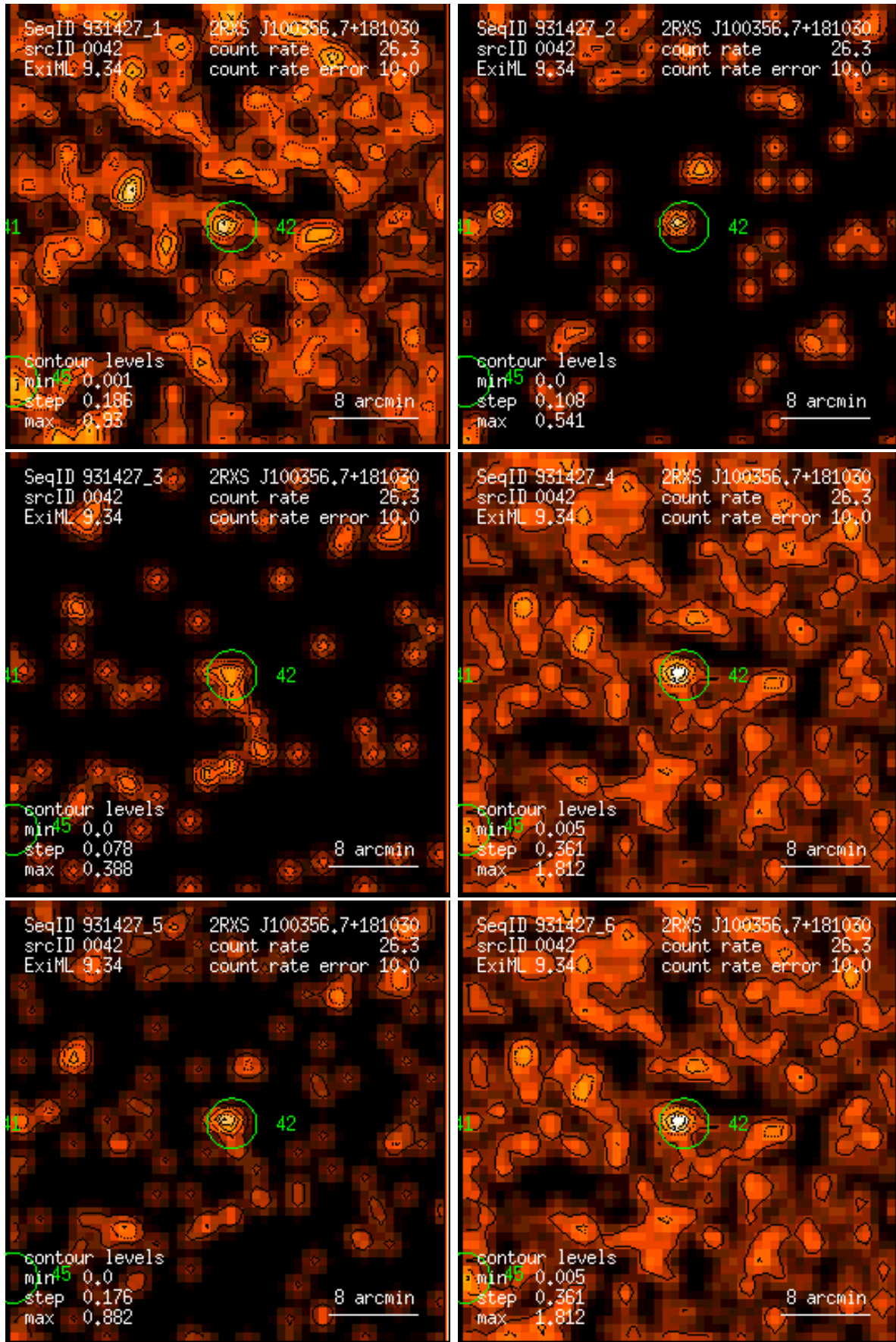
Figure 42: RASS 931427: detection 0042: band rate images, Gaussian filter: (1) PSPC channels 11 – 41, (2) 52 – 90, (3) 91 – 201, (4) 11 – 235, (5) 52 – 201, (6) 11 – 201. Broad band rates in counts/ks. Band rate contour levels in counts/ks/arcmin 2 .
