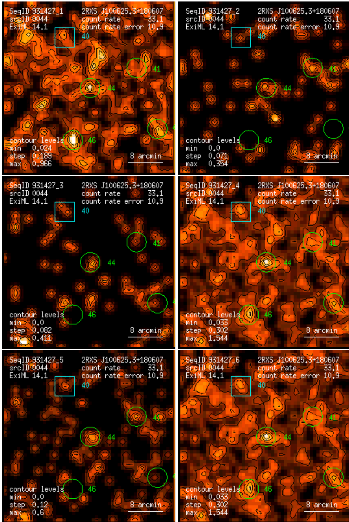
Figure 44: RASS 931427: detection 0044: band rate images, Gaussian filter: (1) PSPC channels 11 – 41, (2) 52 – 90, (3) 91 – 201, (4) 11 – 235, (5) 52 – 201, (6) 11 – 201. Broad band rates in counts/ks. Band rate contour levels in counts/ks/arcmin 2 .
