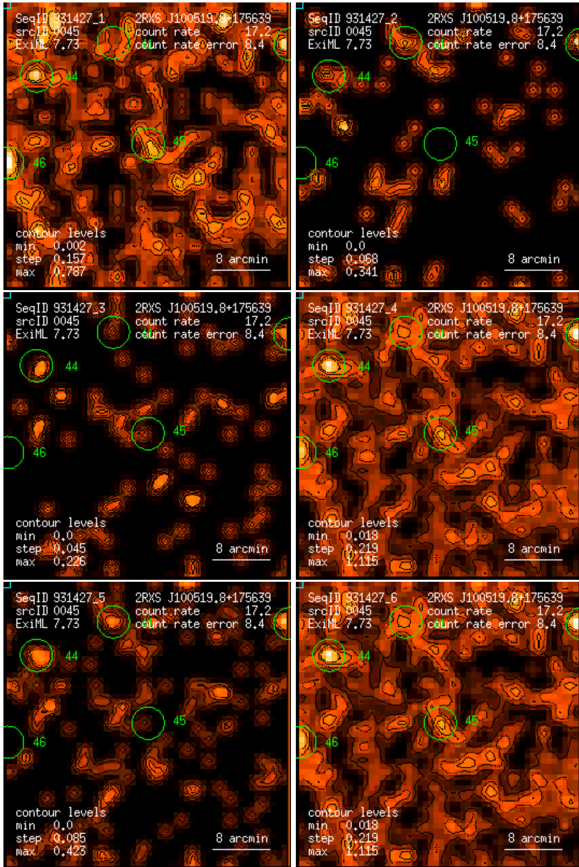
Figure 45: RASS 931427: detection 0045: band rate images, Gaussian filter: (1) PSPC channels 11 – 41, (2) 52 – 90, (3) 91 – 201, (4) 11 – 235, (5) 52 – 201, (6) 11 – 201. Broad band rates in counts/ks. Band rate contour levels in counts/ks/arcmin 2 .
