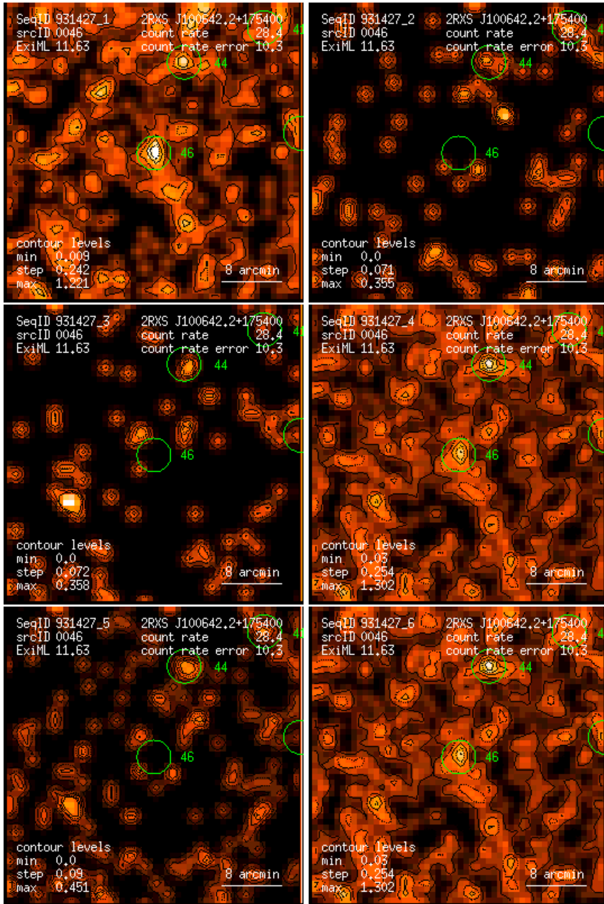
Figure 46: RASS 931427: detection 0046: band rate images, Gaussian filter: (1) PSPC channels 11 – 41, (2) 52 – 90, (3) 91 – 201, (4) 11 – 235, (5) 52 – 201, (6) 11 – 201. Broad band rates in counts/ks. Band rate contour levels in counts/ks/arcmin 2 .
