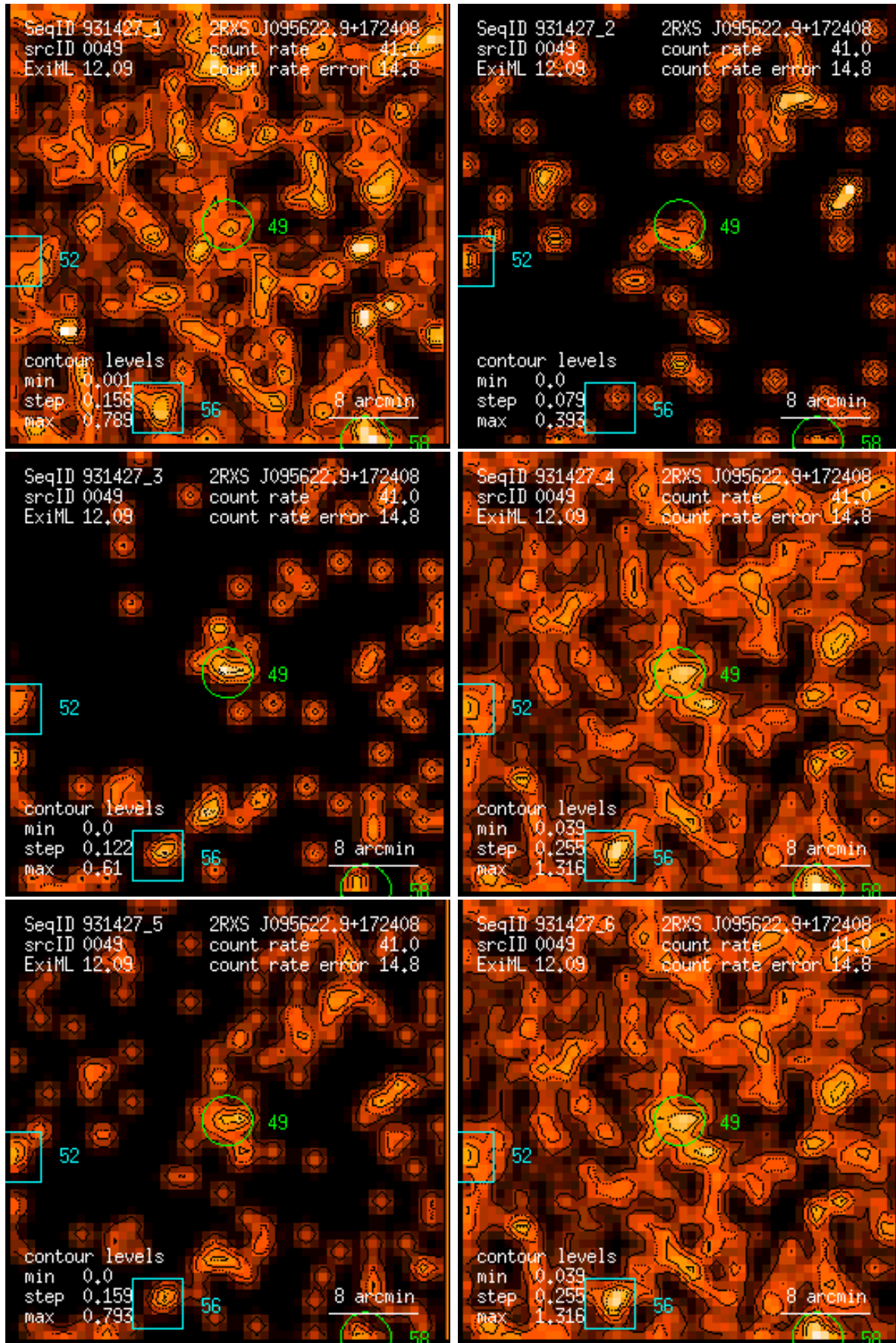
Figure 49: RASS 931427: detection 0049: band rate images, Gaussian filter: (1) PSPC channels 11 – 41, (2) 52 – 90, (3) 91 – 201, (4) 11 – 235, (5) 52 – 201, (6) 11 – 201. Broad band rates in counts/ks. Band rate contour levels in counts/ks/arcmin 2 .
