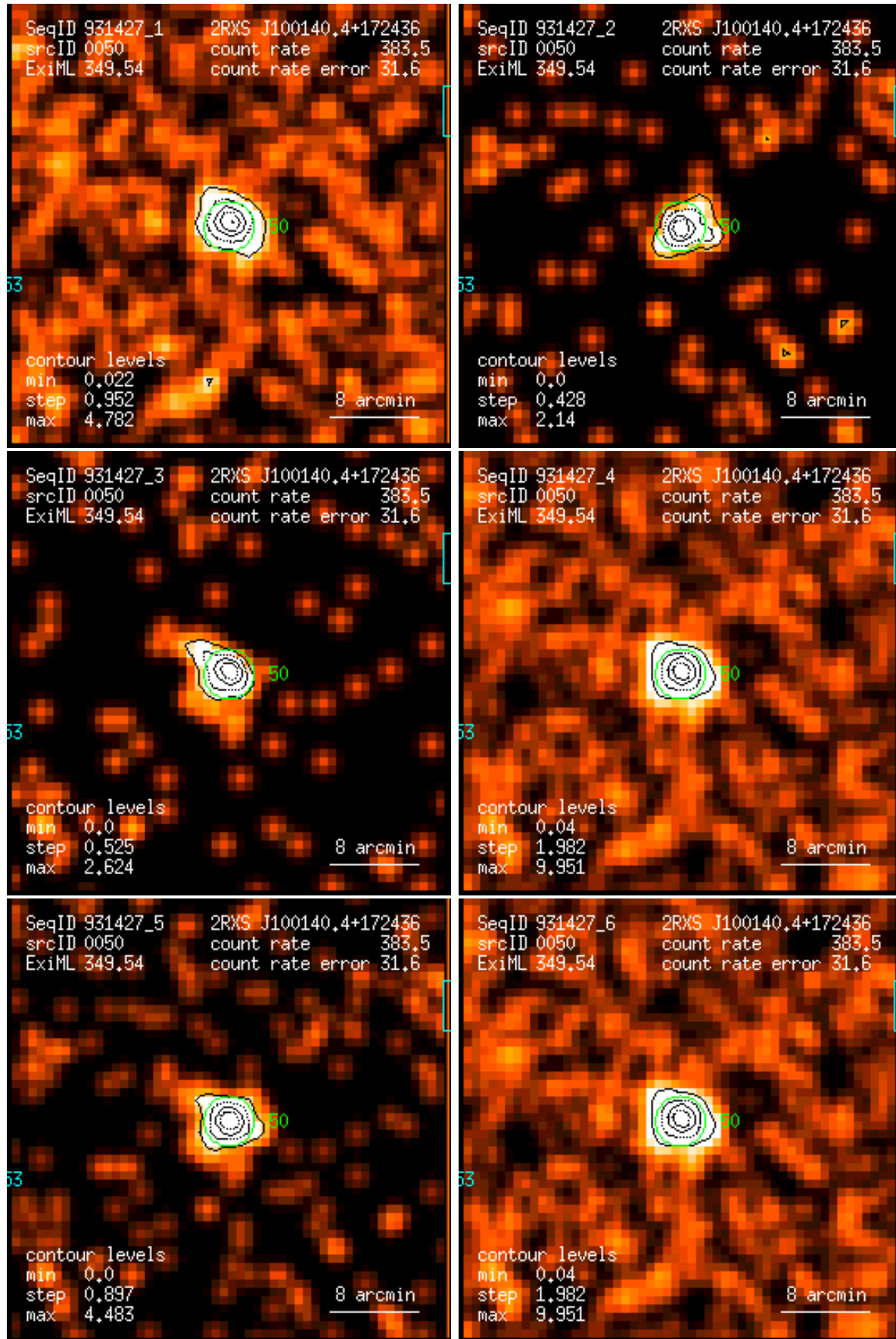
Figure 50: RASS 931427: detection 0050: band rate images, Gaussian filter: (1) PSPC channels 11 – 41, (2) 52 – 90, (3) 91 – 201, (4) 11 – 235, (5) 52 – 201, (6) 11 – 201. Broad band rates in counts/ks. Band rate contour levels in counts/ks/arcmin 2 .
