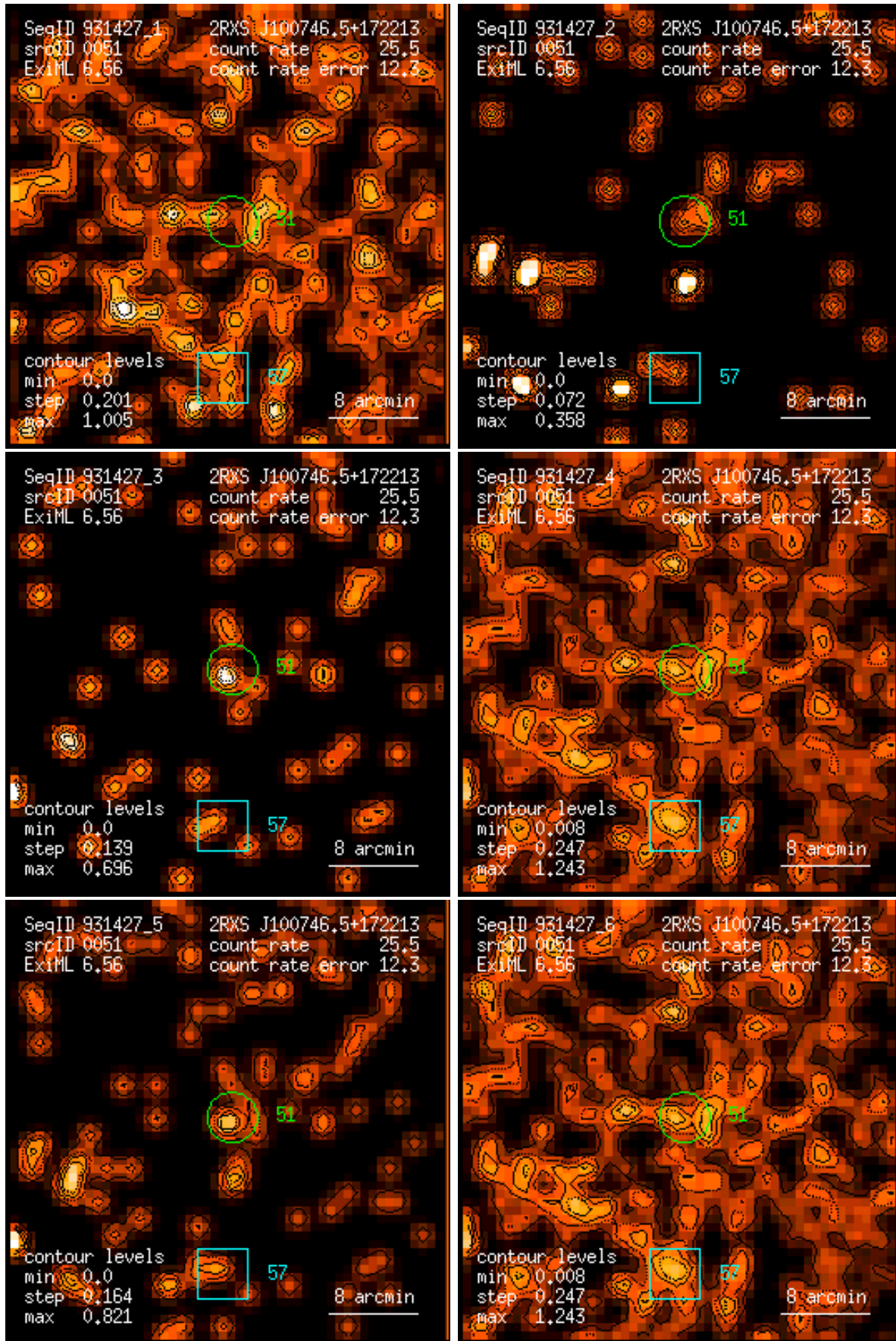
Figure 51: RASS 931427: detection 0051: band rate images, Gaussian filter: (1) PSPC channels 11 – 41, (2) 52 – 90, (3) 91 – 201, (4) 11 – 235, (5) 52 – 201, (6) 11 – 201. Broad band rates in counts/ks. Band rate contour levels in counts/ks/arcmin 2 .
