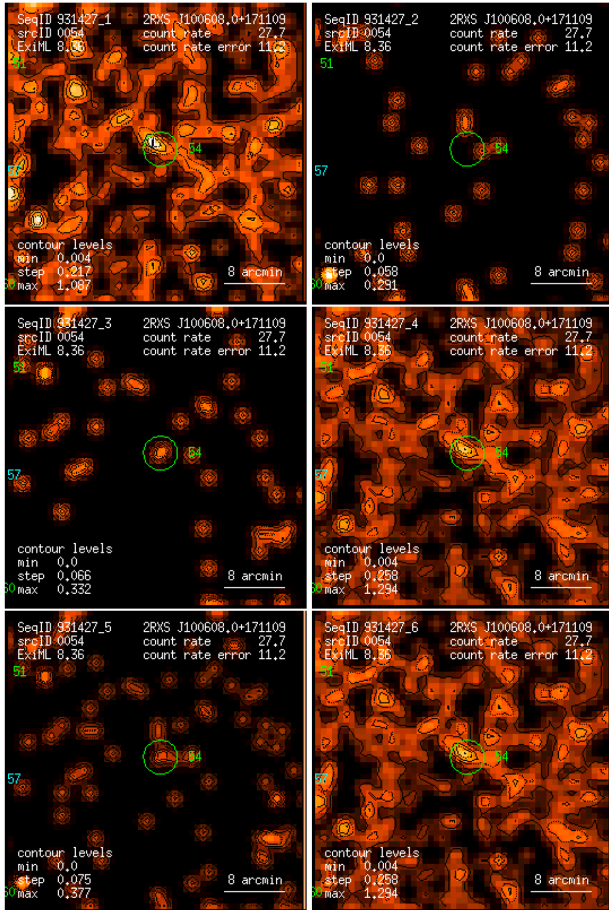
Figure 54: RASS 931427: detection 0054: band rate images, Gaussian filter: (1) PSPC channels 11 – 41, (2) 52 – 90, (3) 91 – 201, (4) 11 – 235, (5) 52 – 201, (6) 11 – 201. Broad band rates in counts/ks. Band rate contour levels in counts/ks/arcmin 2 .
