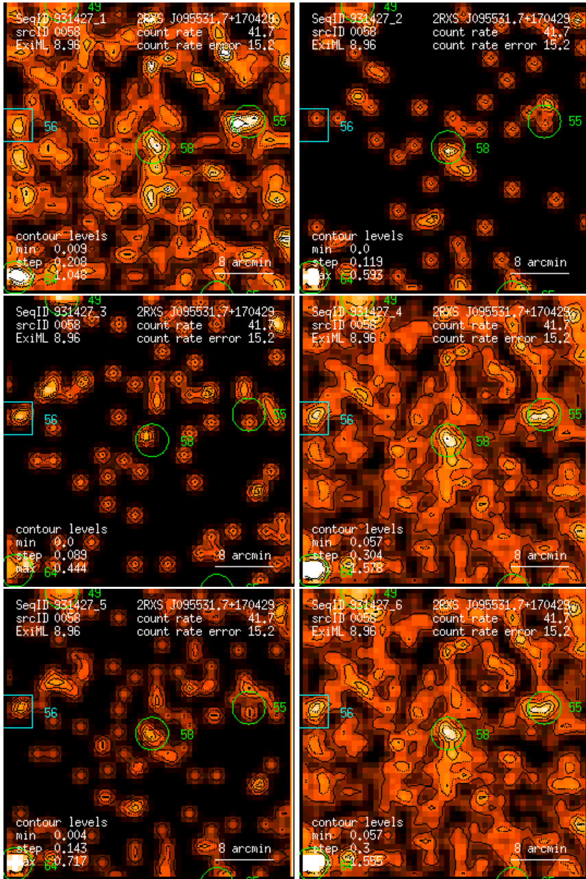
Figure 58: RASS 931427: detection 0058: band rate images, Gaussian filter: (1) PSPC channels 11 – 41, (2) 52 – 90, (3) 91 – 201, (4) 11 – 235, (5) 52 – 201, (6) 11 – 201. Broad band rates in counts/ks. Band rate contour levels in counts/ks/arcmin 2 .
