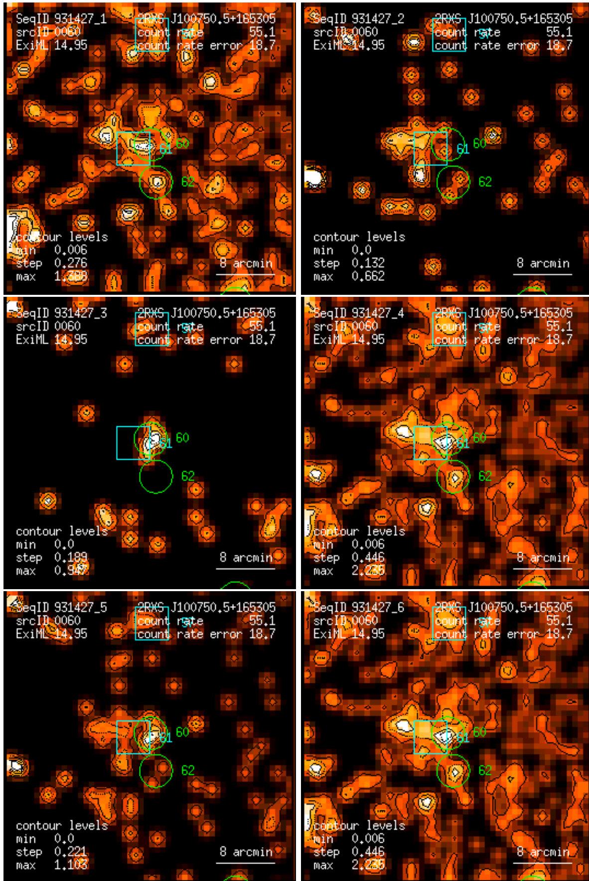
Figure 60: RASS 931427: detection 0060: band rate images, Gaussian filter: (1) PSPC channels 11 – 41, (2) 52 – 90, (3) 91 – 201, (4) 11 – 235, (5) 52 – 201, (6) 11 – 201. Broad band rates in counts/ks. Band rate contour levels in counts/ks/arcmin 2 .
