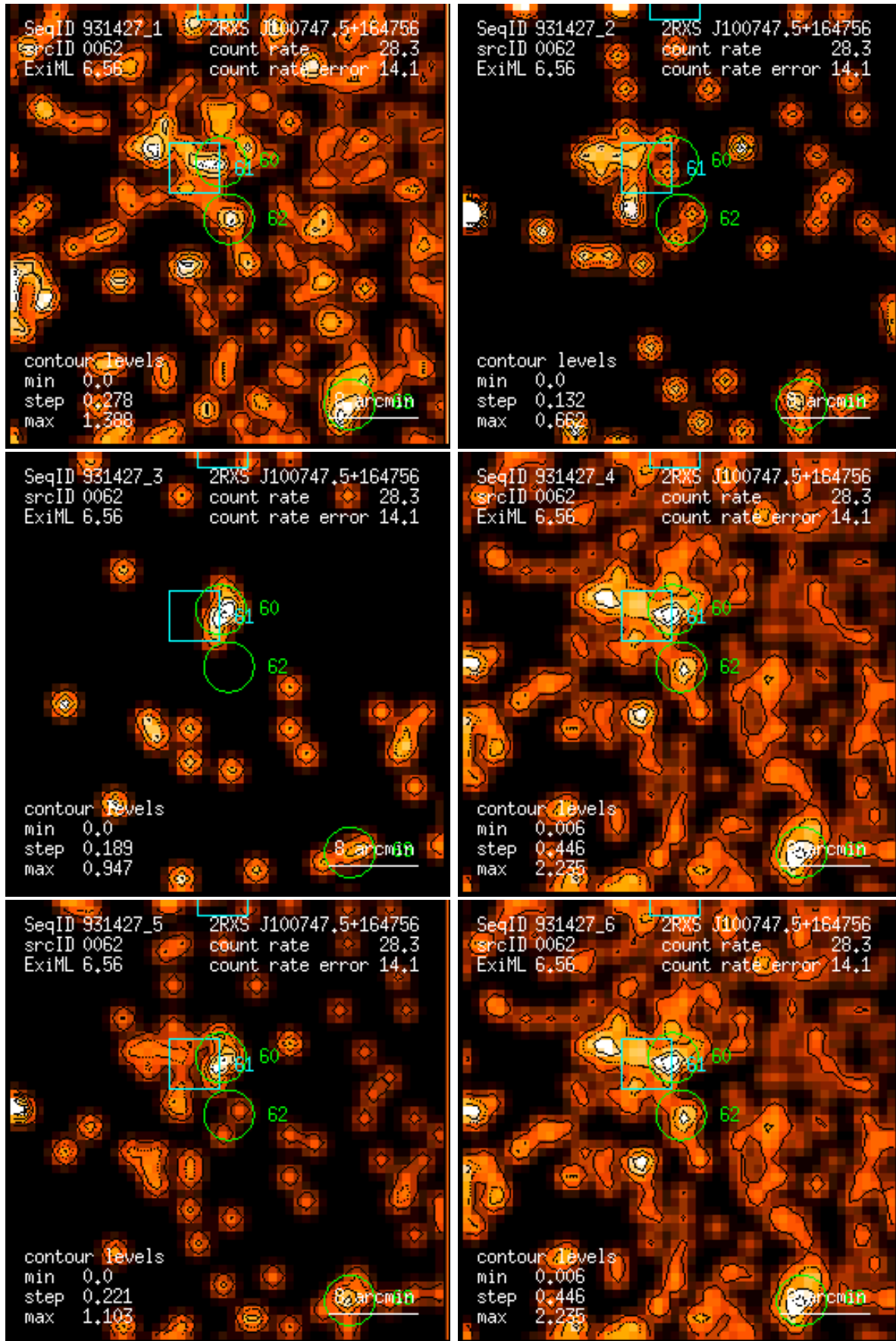
Figure 62: RASS 931427: detection 0062: band rate images, Gaussian filter: (1) PSPC channels 11 – 41, (2) 52 – 90, (3) 91 – 201, (4) 11 – 235, (5) 52 – 201, (6) 11 – 201. Broad band rates in counts/ks. Band rate contour levels in counts/ks/arcmin 2 .
