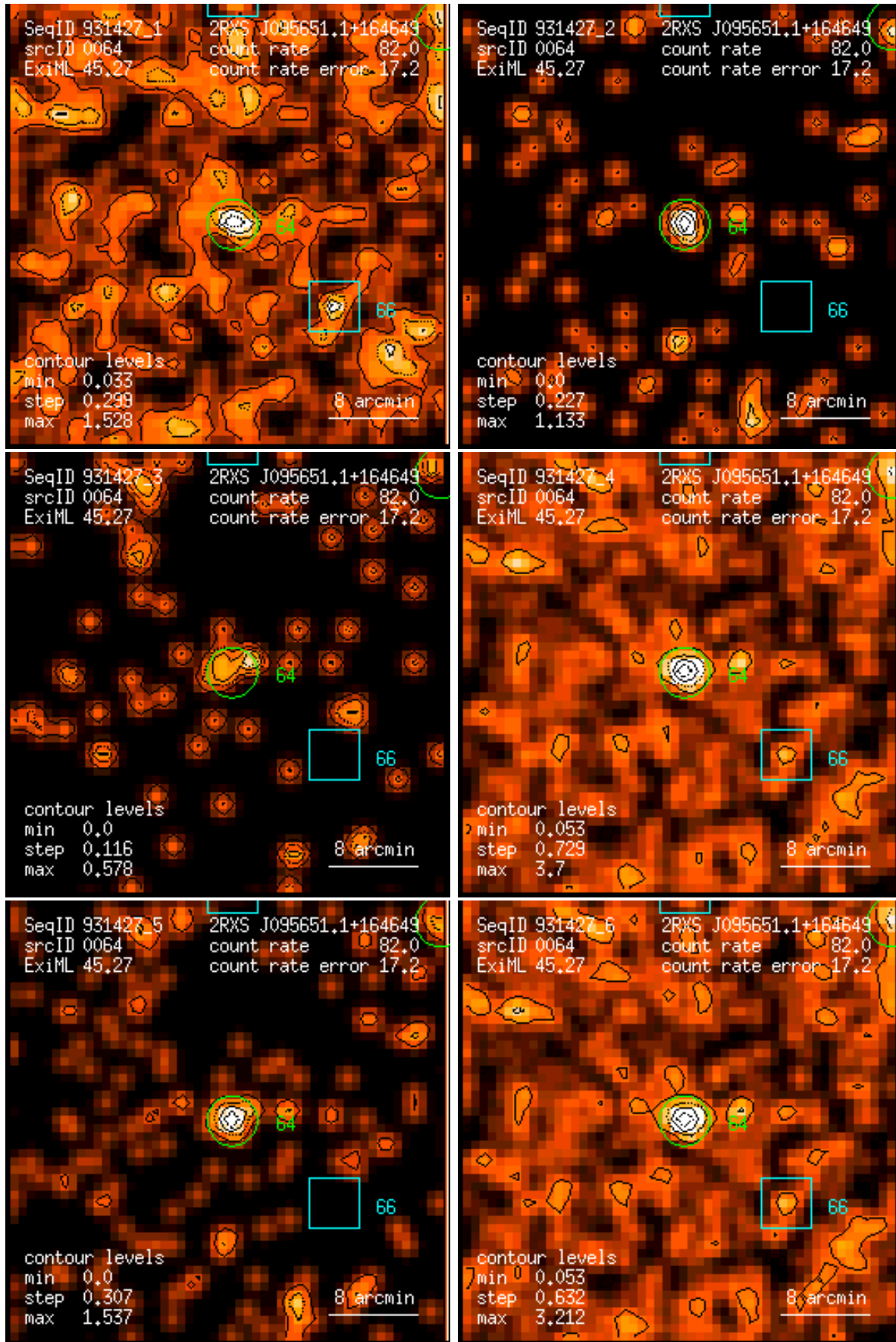
Figure 64: RASS 931427: detection 0064: band rate images, Gaussian filter: (1) PSPC channels 11 – 41, (2) 52 – 90, (3) 91 – 201, (4) 11 – 235, (5) 52 – 201, (6) 11 – 201. Broad band rates in counts/ks. Band rate contour levels in counts/ks/arcmin 2 .
