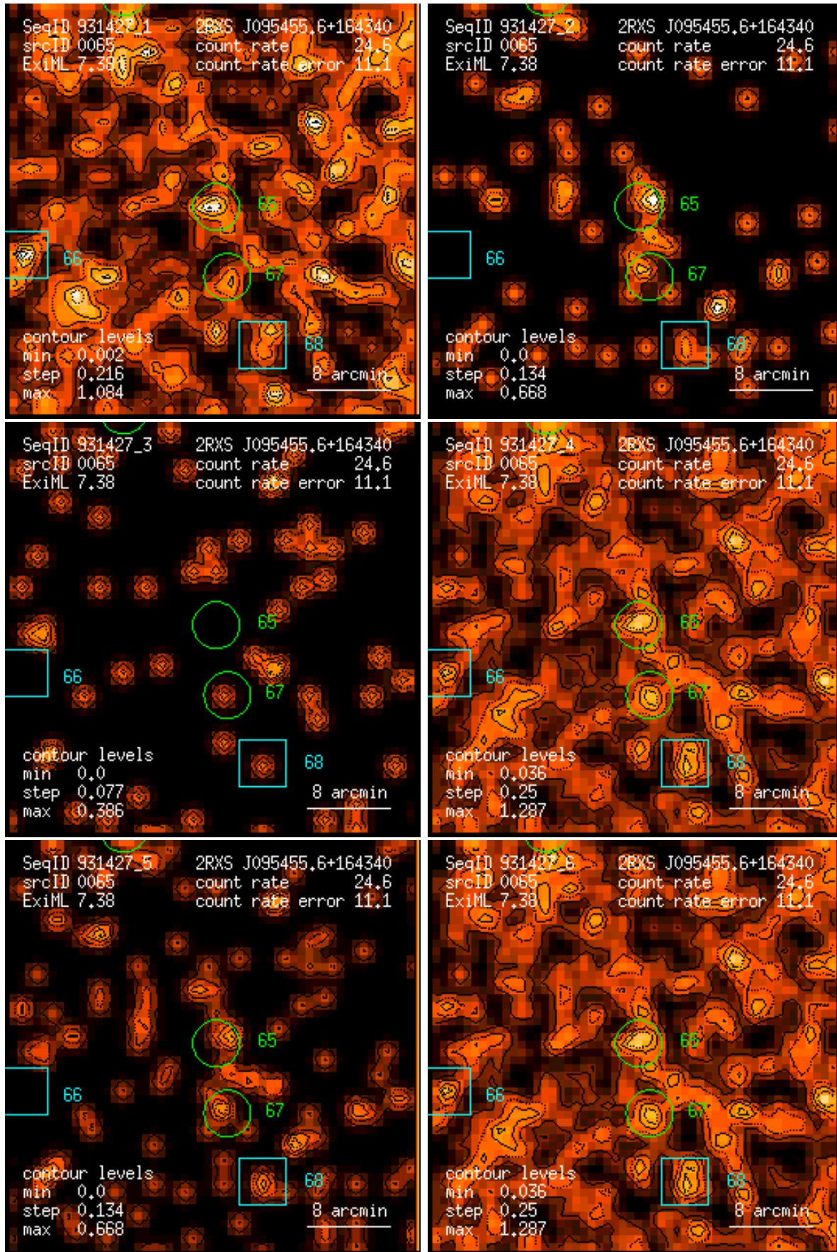
Figure 65: RASS 931427: detection 0065: band rate images, Gaussian filter: (1) PSPC channels 11 – 41, (2) 52 – 90, (3) 91 – 201, (4) 11 – 235, (5) 52 – 201, (6) 11 – 201. Broad band rates in counts/ks. Band rate contour levels in counts/ks/arcmin 2 .
