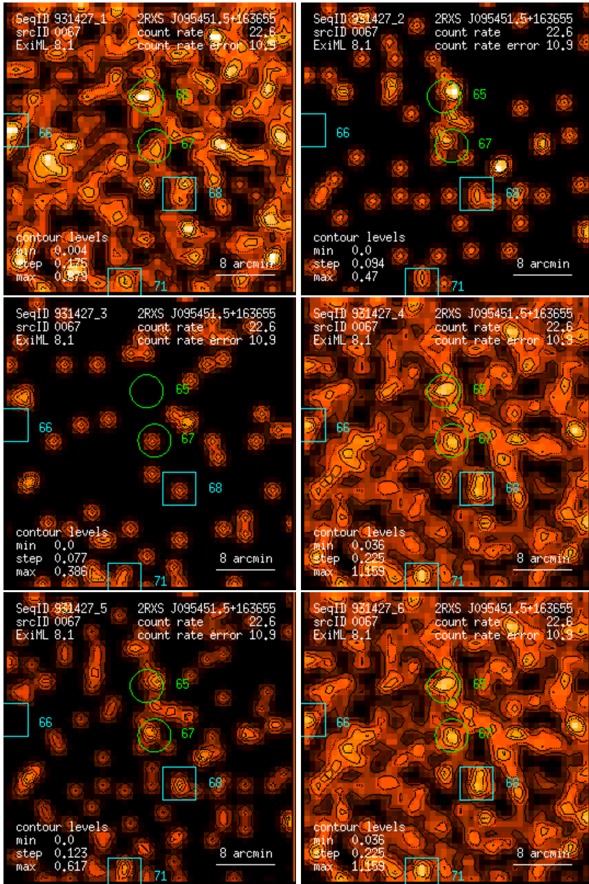
Figure 67: RASS 931427: detection 0067: band rate images, Gaussian filter: (1) PSPC channels 11 – 41, (2) 52 – 90, (3) 91 – 201, (4) 11 – 235, (5) 52 – 201, (6) 11 – 201. Broad band rates in counts/ks. Band rate contour levels in counts/ks/arcmin 2 .
