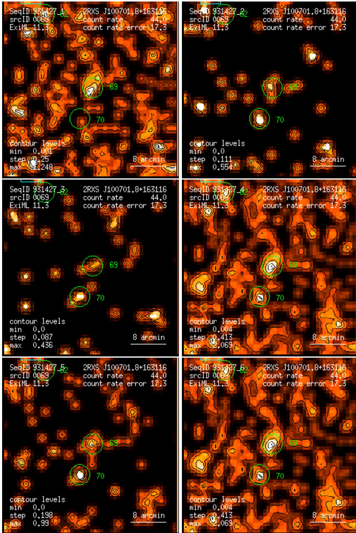
Figure 69: RASS 931427: detection 0069: band rate images, Gaussian filter: (1) PSPC channels 11 – 41, (2) 52 – 90, (3) 91 – 201, (4) 11 – 235, (5) 52 – 201, (6) 11 – 201. Broad band rates in counts/ks. Band rate contour levels in counts/ks/arcmin 2 .
