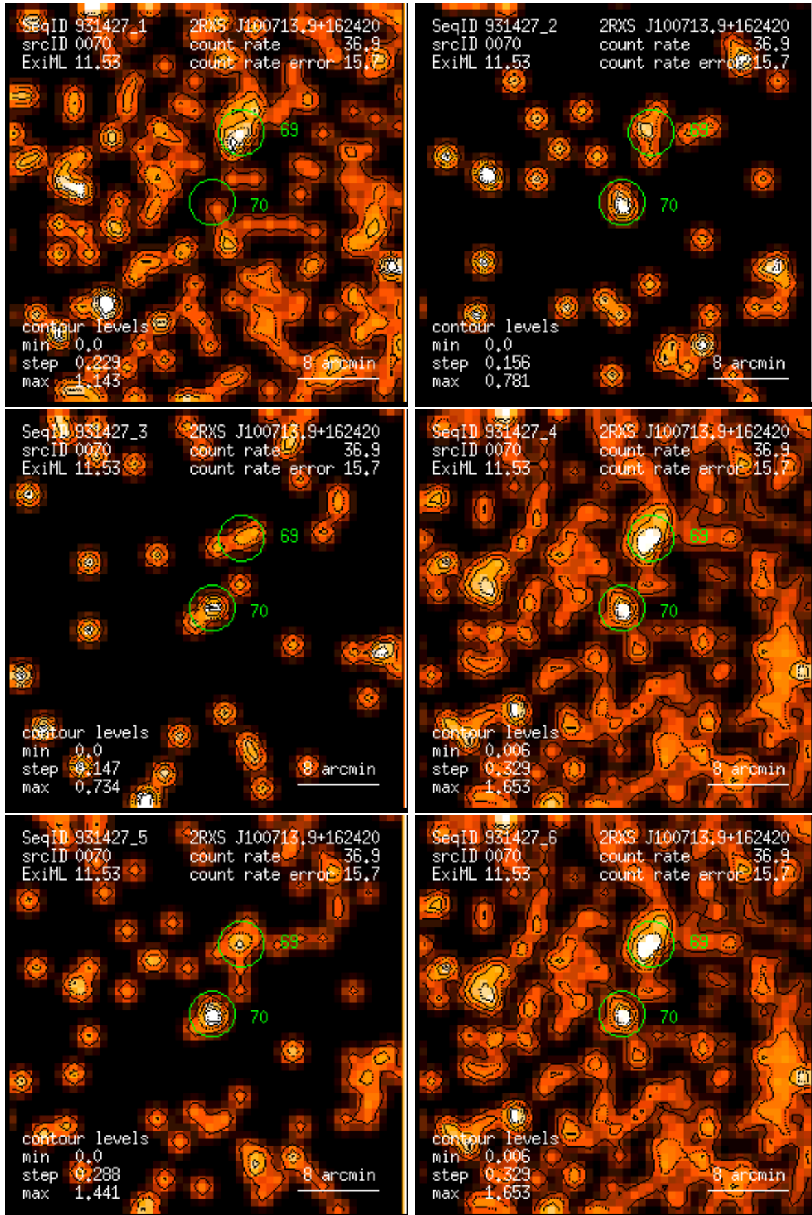
Figure 70: RASS 931427: detection 0070: band rate images, Gaussian filter: (1) PSPC channels 11 – 41, (2) 52 – 90, (3) 91 – 201, (4) 11 – 235, (5) 52 – 201, (6) 11 – 201. Broad band rates in counts/ks. Band rate contour levels in counts/ks/arcmin 2 .
