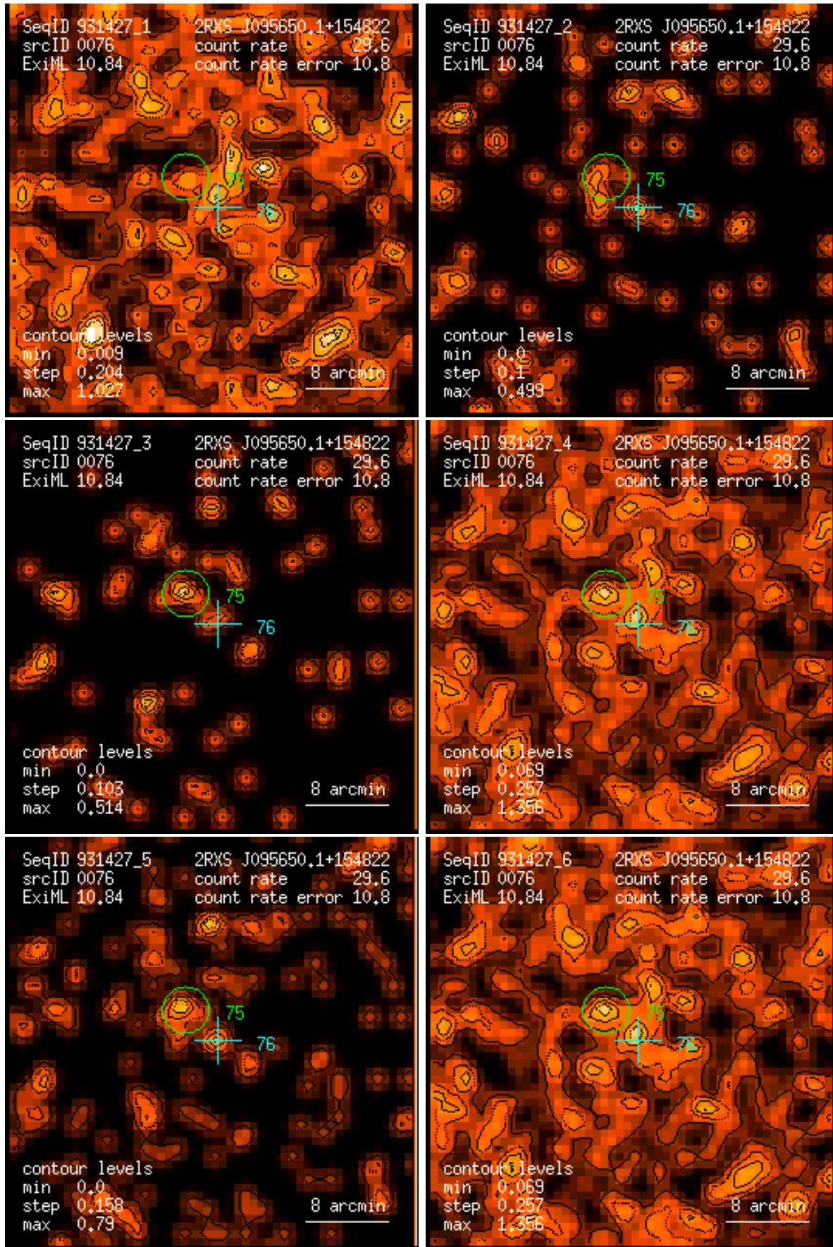
Figure 76: RASS 931427: detection 0076: band rate images, Gaussian filter: (1) PSPC channels 11 – 41, (2) 52 – 90, (3) 91 – 201, (4) 11 – 235, (5) 52 – 201, (6) 11 – 201. Broad band rates in counts/ks. Band rate contour levels in counts/ks/arcmin 2 .
