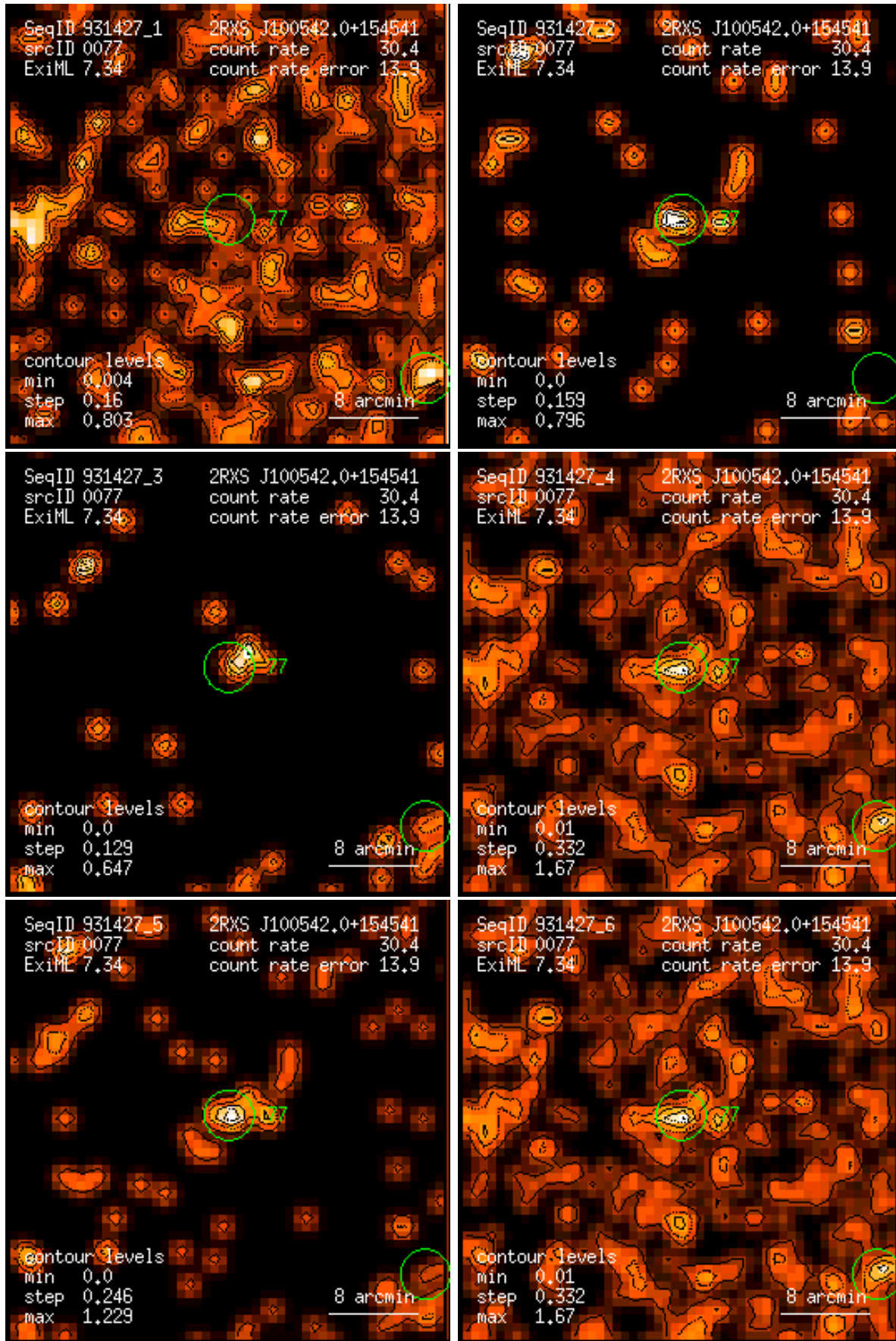
Figure 77: RASS 931427: detection 0077: band rate images, Gaussian filter: (1) PSPC channels 11 – 41, (2) 52 – 90, (3) 91 – 201, (4) 11 – 235, (5) 52 – 201, (6) 11 – 201. Broad band rates in counts/ks. Band rate contour levels in counts/ks/arcmin 2 .
