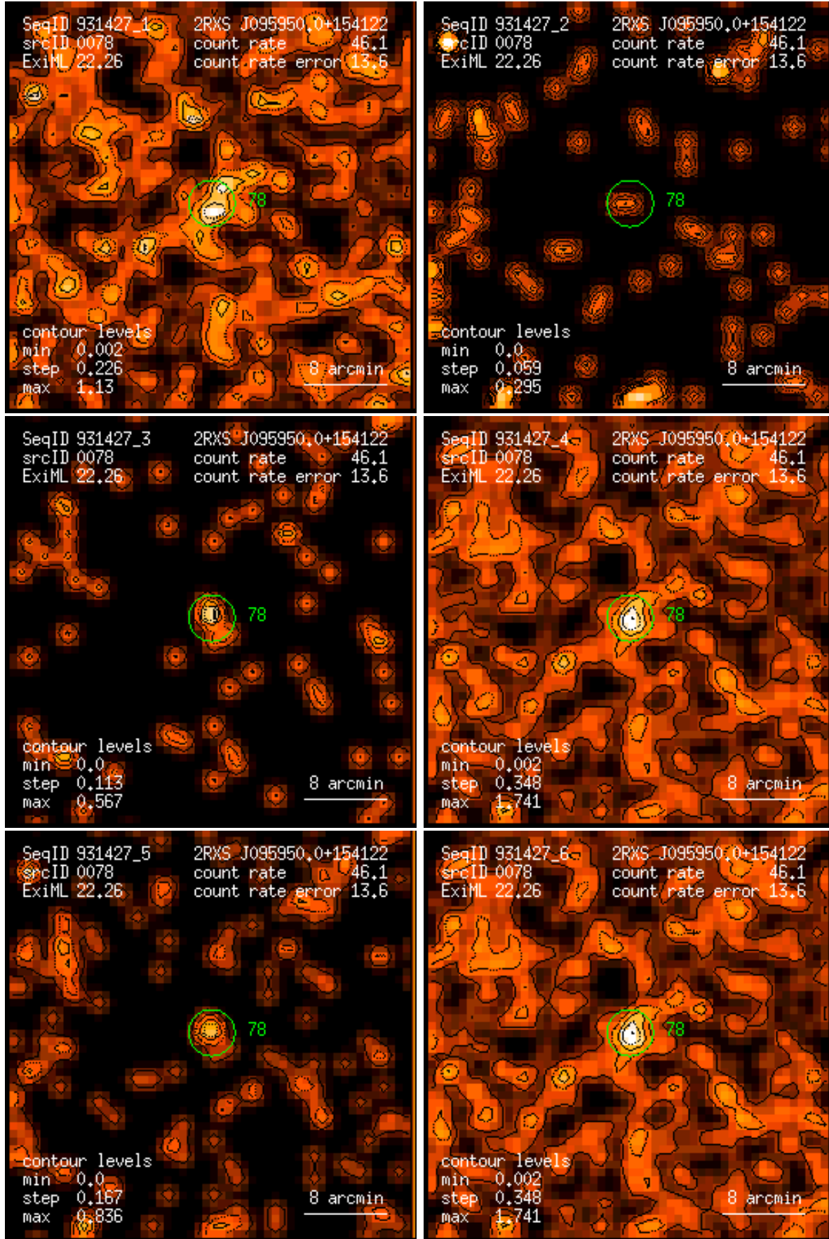
Figure 78: RASS 931427: detection 0078: band rate images, Gaussian filter: (1) PSPC channels 11 – 41, (2) 52 – 90, (3) 91 – 201, (4) 11 – 235, (5) 52 – 201, (6) 11 – 201. Broad band rates in counts/ks. Band rate contour levels in counts/ks/arcmin 2 .
