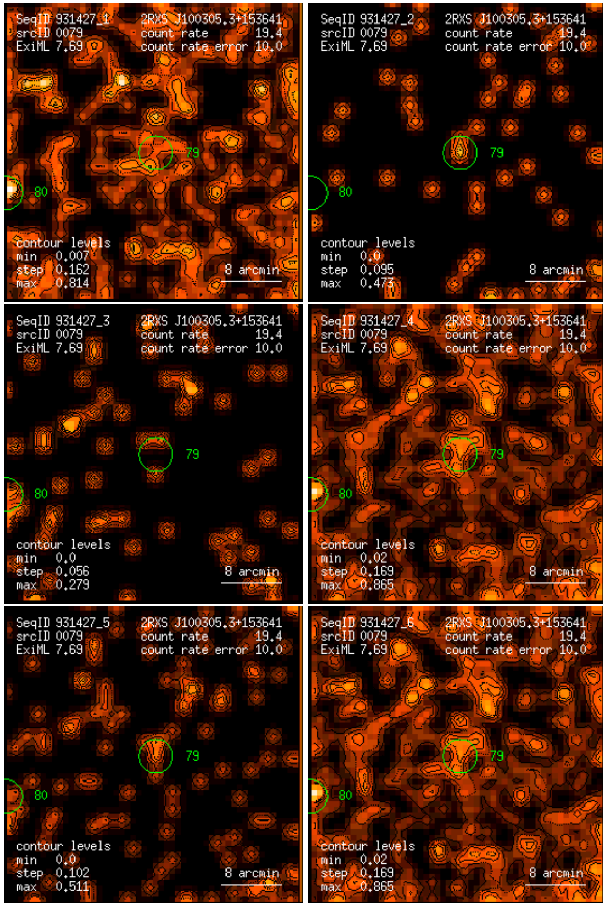
Figure 79: RASS 931427: detection 0079: band rate images, Gaussian filter: (1) PSPC channels 11 – 41, (2) 52 – 90, (3) 91 – 201, (4) 11 – 235, (5) 52 – 201, (6) 11 – 201. Broad band rates in counts/ks. Band rate contour levels in counts/ks/arcmin 2 .
