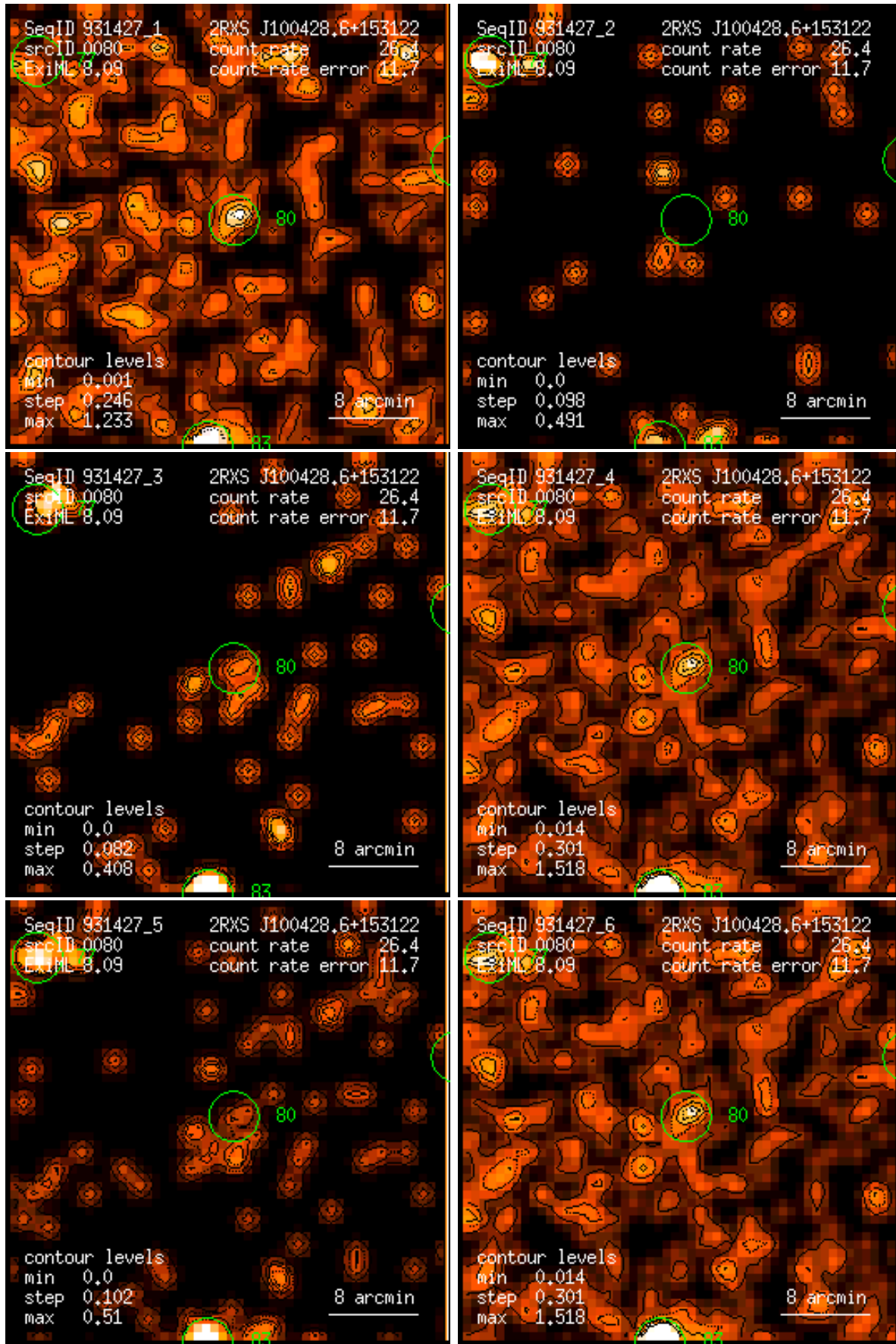
Figure 80: RASS 931427: detection 0080: band rate images, Gaussian filter: (1) PSPC channels 11 – 41, (2) 52 – 90, (3) 91 – 201, (4) 11 – 235, (5) 52 – 201, (6) 11 – 201. Broad band rates in counts/ks. Band rate contour levels in counts/ks/arcmin 2 .
