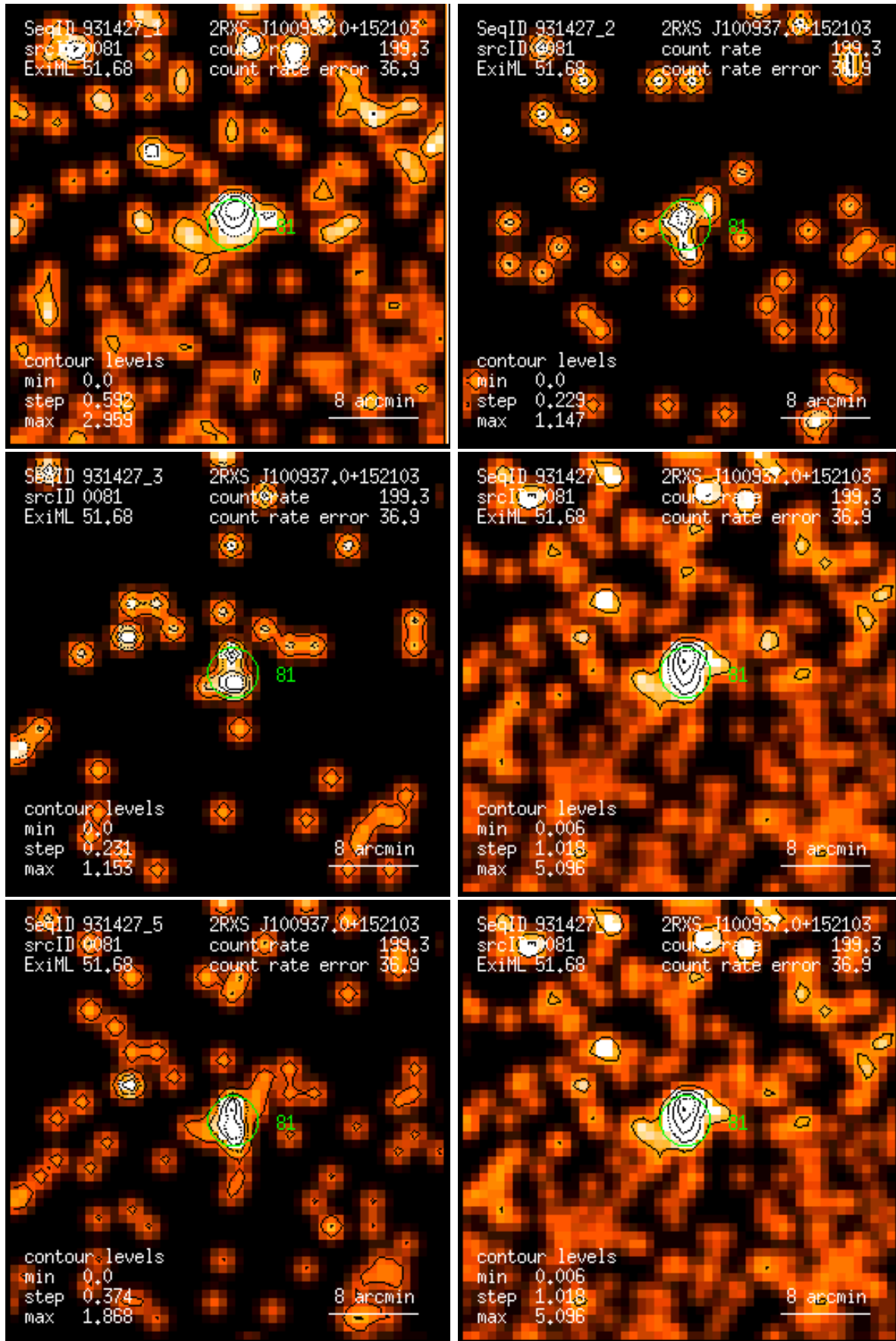
Figure 81: RASS 931427: detection 0081: band rate images, Gaussian filter: (1) PSPC channels 11 – 41, (2) 52 – 90, (3) 91 – 201, (4) 11 – 235, (5) 52 – 201, (6) 11 – 201. Broad band rates in counts/ks. Band rate contour levels in counts/ks/arcmin 2 .
