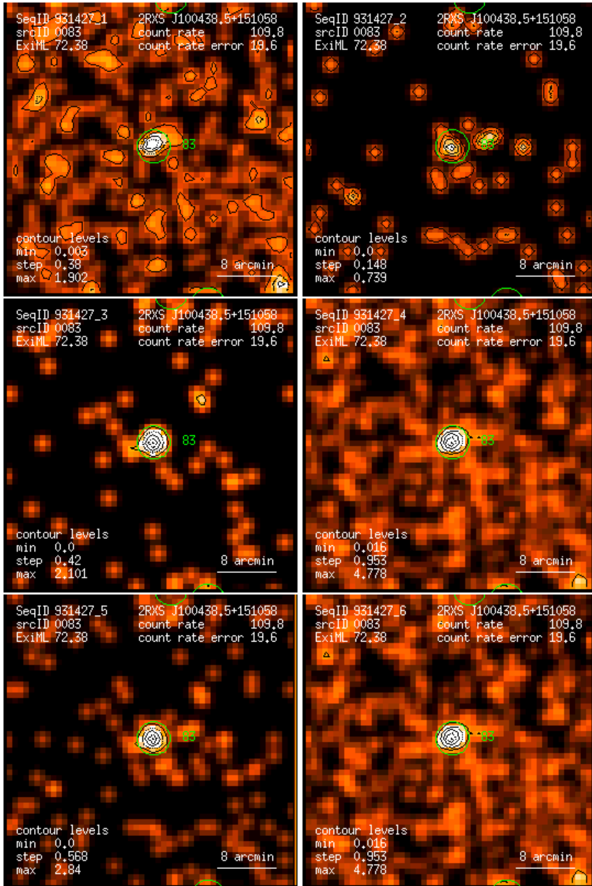
Figure 83: RASS 931427: detection 0083: band rate images, Gaussian filter: (1) PSPC channels 11 – 41, (2) 52 – 90, (3) 91 – 201, (4) 11 – 235, (5) 52 – 201, (6) 11 – 201. Broad band rates in counts/ks. Band rate contour levels in counts/ks/arcmin 2 .
