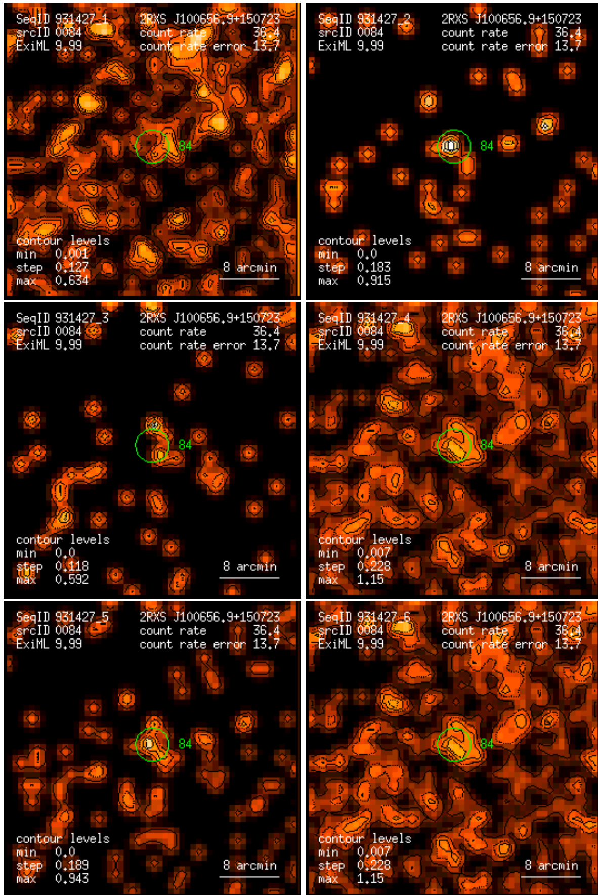
Figure 84: RASS 931427: detection 0084: band rate images, Gaussian filter: (1) PSPC channels 11 – 41, (2) 52 – 90, (3) 91 – 201, (4) 11 – 235, (5) 52 – 201, (6) 11 – 201. Broad band rates in counts/ks. Band rate contour levels in counts/ks/arcmin 2 .
