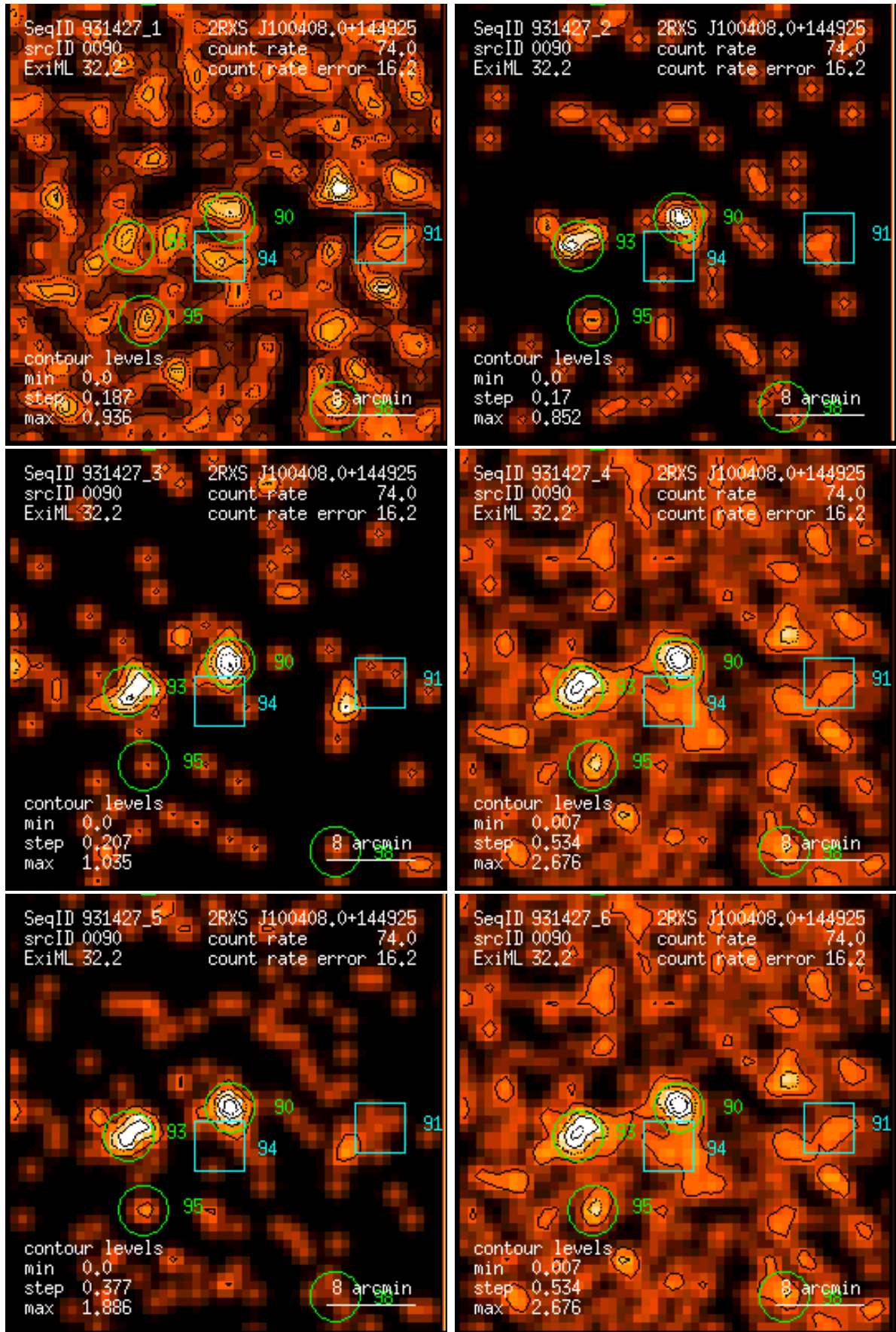
Figure 90: RASS 931427: detection 0090: band rate images, Gaussian filter: (1) PSPC channels 11 – 41, (2) 52 – 90, (3) 91 – 201, (4) 11 – 235, (5) 52 – 201, (6) 11 – 201. Broad band rates in counts/ks. Band rate contour levels in counts/ks/arcmin 2 .
