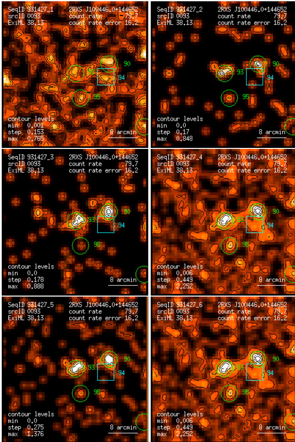
Figure 93: RASS 931427: detection 0093: band rate images, Gaussian filter: (1) PSPC channels 11 – 41, (2) 52 – 90, (3) 91 – 201, (4) 11 – 235, (5) 52 – 201, (6) 11 – 201. Broad band rates in counts/ks. Band rate contour levels in counts/ks/arcmin 2 .
