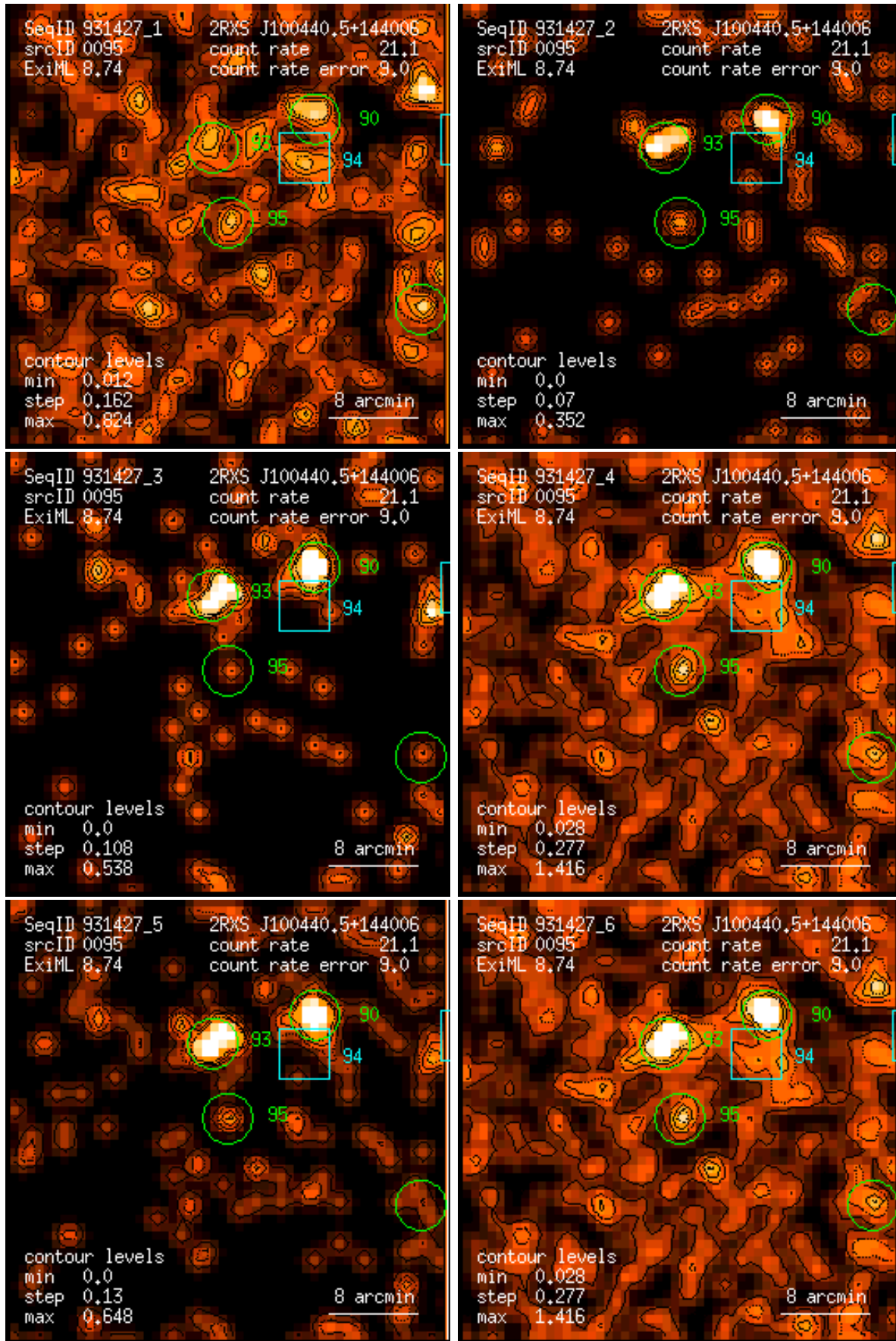
Figure 95: RASS 931427: detection 0095: band rate images, Gaussian filter: (1) PSPC channels 11 – 41, (2) 52 – 90, (3) 91 – 201, (4) 11 – 235, (5) 52 – 201, (6) 11 – 201. Broad band rates in counts/ks. Band rate contour levels in counts/ks/arcmin 2 .
