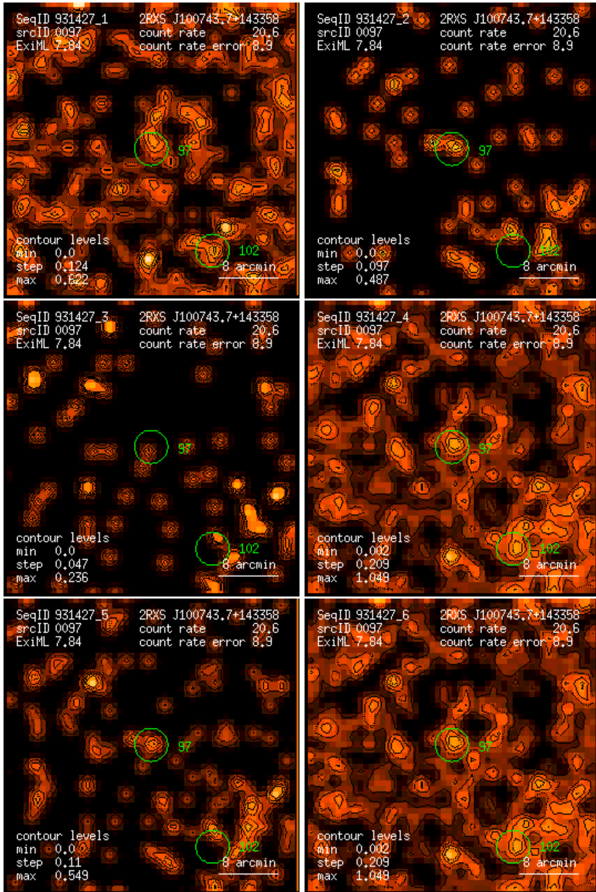
Figure 97: RASS 931427: detection 0097: band rate images, Gaussian filter: (1) PSPC channels 11 – 41, (2) 52 – 90, (3) 91 – 201, (4) 11 – 235, (5) 52 – 201, (6) 11 – 201. Broad band rates in counts/ks. Band rate contour levels in counts/ks/arcmin 2 .
