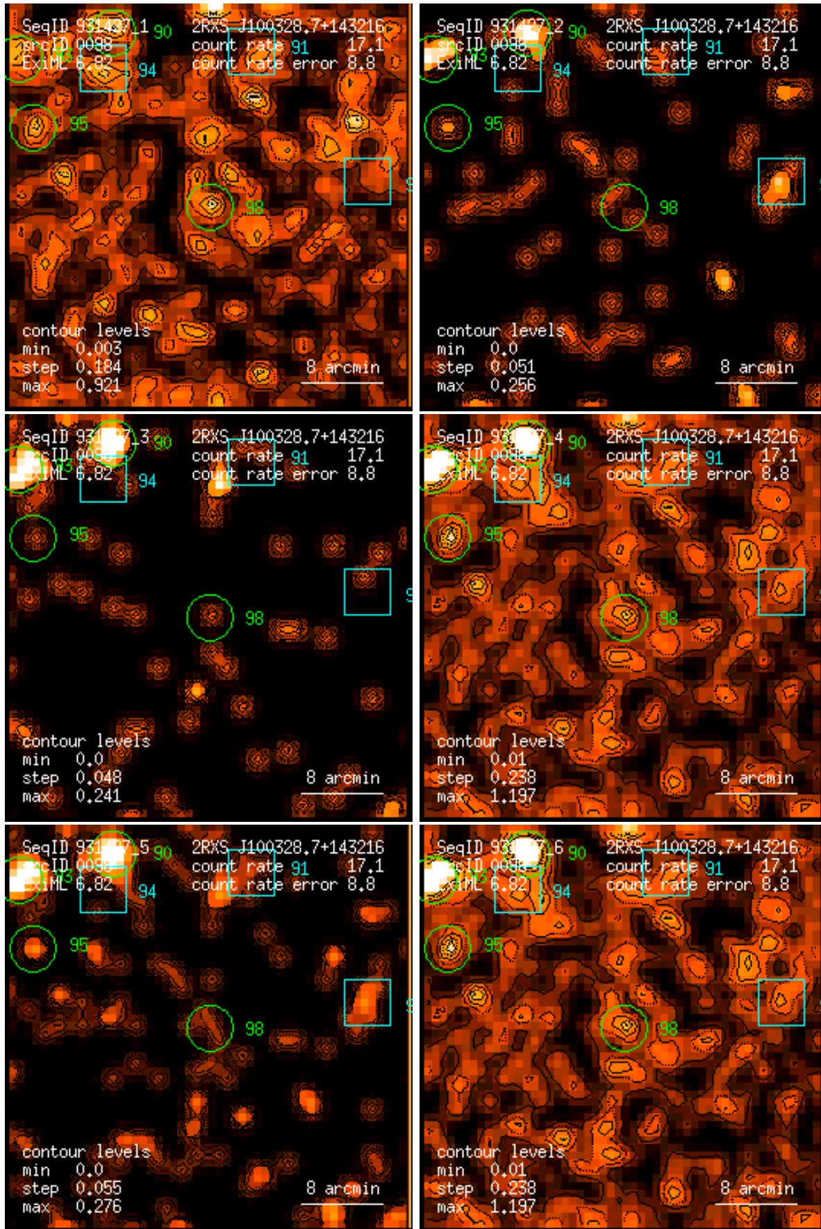
Figure 98: RASS 931427: detection 0098: band rate images, Gaussian filter: (1) PSPC channels 11 – 41, (2) 52 – 90, (3) 91 – 201, (4) 11 – 235, (5) 52 – 201, (6) 11 – 201. Broad band rates in counts/ks. Band rate contour levels in counts/ks/arcmin 2 .
