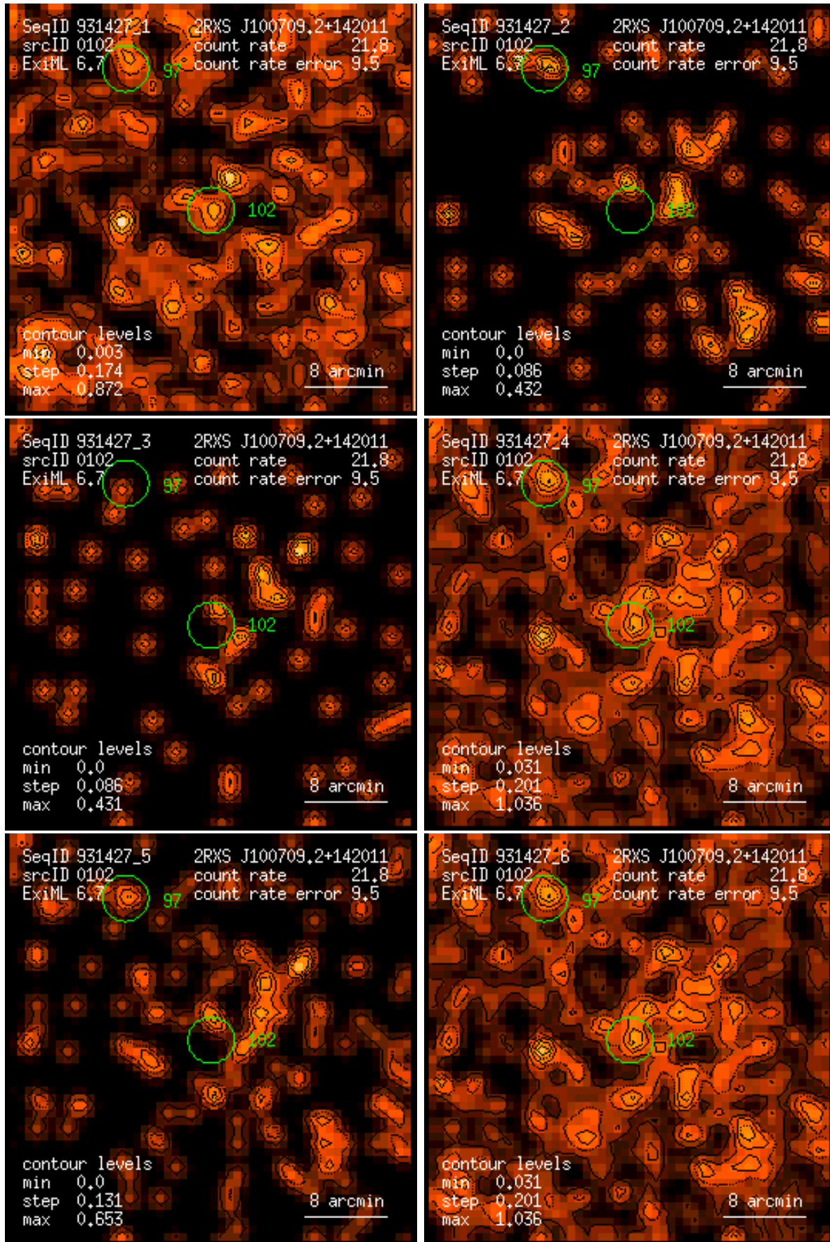
Figure 102: RASS 931427: detection 0102: band rate images, Gaussian filter: (1) PSPC channels 11 – 41, (2) 52 – 90, (3) 91 – 201, (4) 11 – 235, (5) 52 – 201, (6) 11 – 201. Broad band rates in counts/ks. Band rate contour levels in counts/ks/arcmin 2 .
