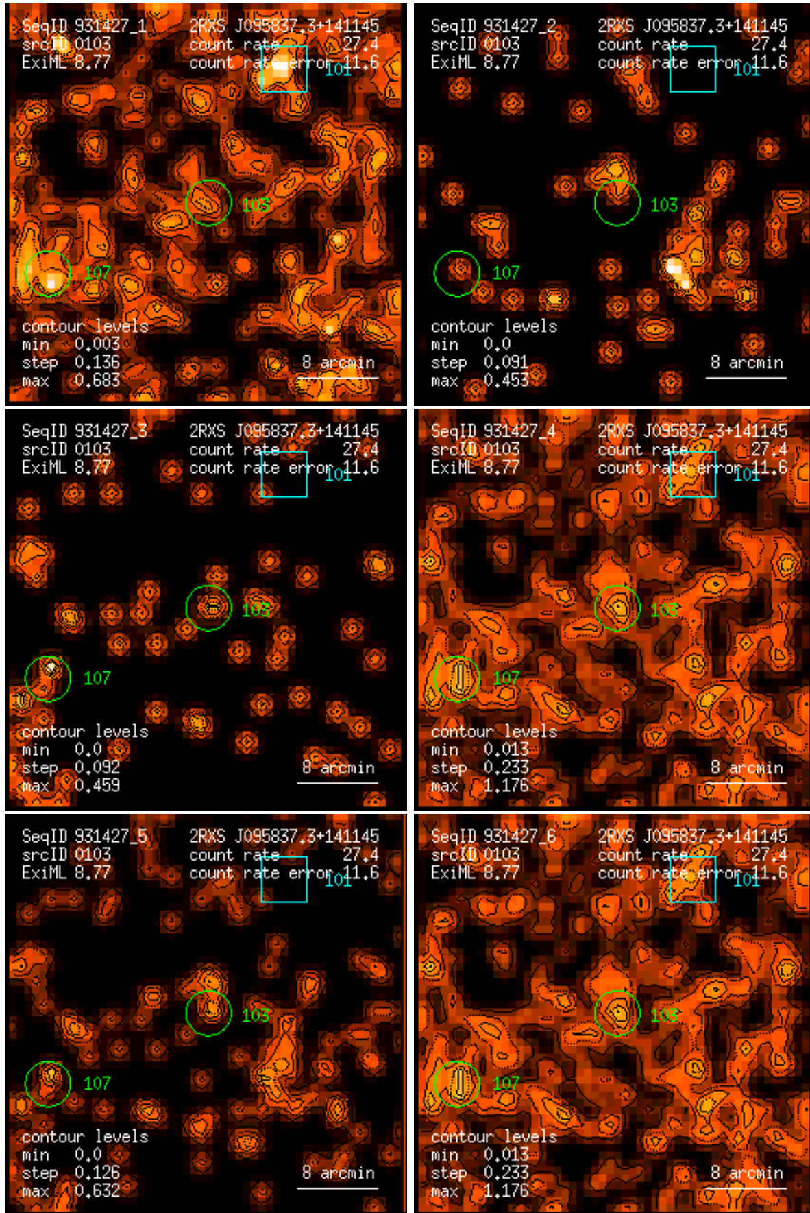
Figure 103: RASS 931427: detection 0103: band rate images, Gaussian filter: (1) PSPC channels 11 – 41, (2) 52 – 90, (3) 91 – 201, (4) 11 – 235, (5) 52 – 201, (6) 11 – 201. Broad band rates in counts/ks. Band rate contour levels in counts/ks/arcmin 2 .
