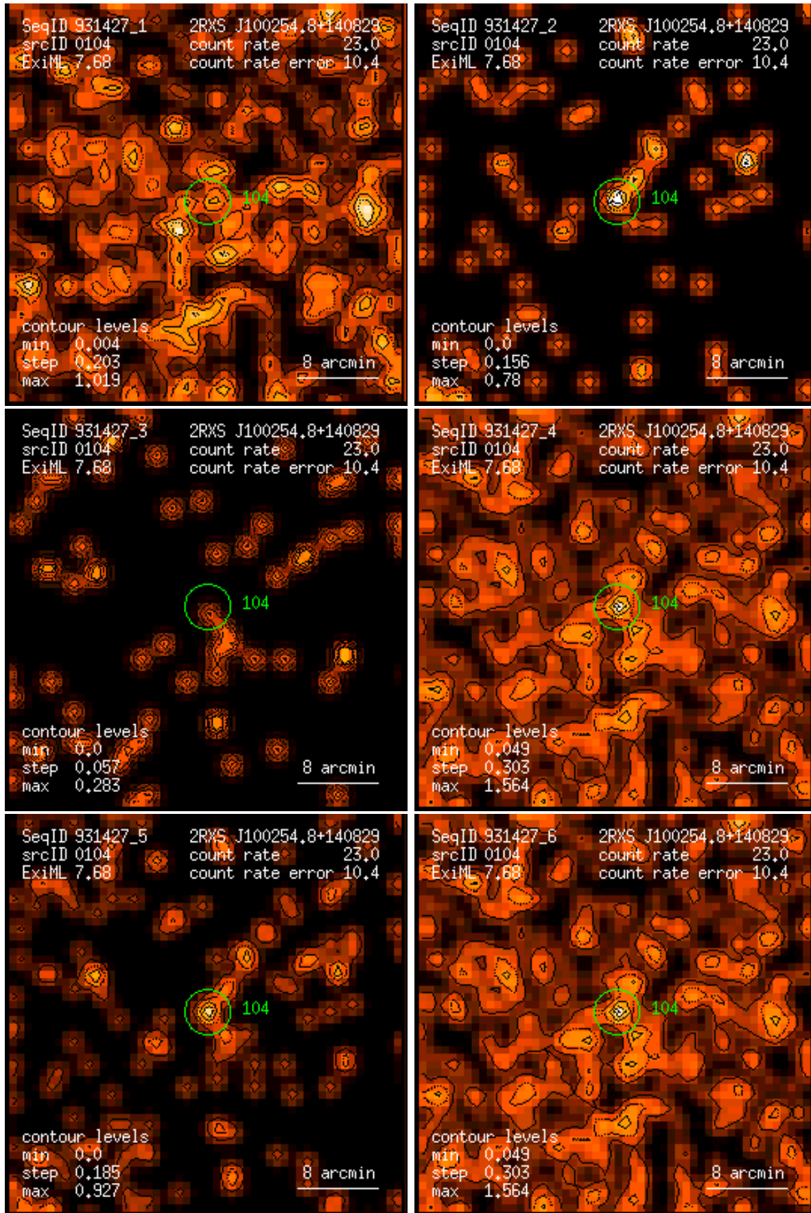
Figure 104: RASS 931427: detection 0104: band rate images, Gaussian filter: (1) PSPC channels 11 – 41, (2) 52 – 90, (3) 91 – 201, (4) 11 – 235, (5) 52 – 201, (6) 11 – 201. Broad band rates in counts/ks. Band rate contour levels in counts/ks/arcmin 2 .
