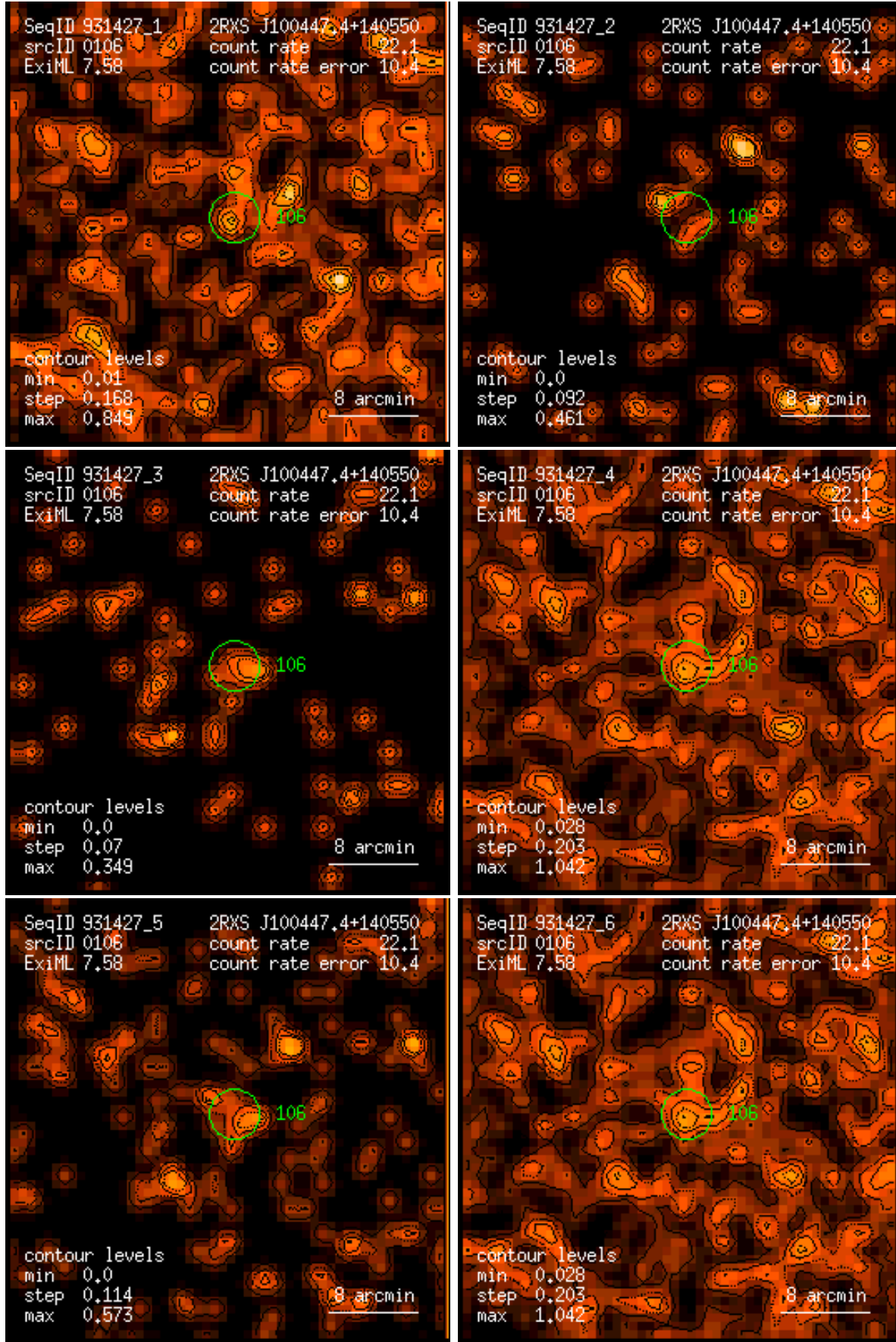
Figure 106: RASS 931427: detection 0106: band rate images, Gaussian filter: (1) PSPC channels 11 – 41, (2) 52 – 90, (3) 91 – 201, (4) 11 – 235, (5) 52 – 201, (6) 11 – 201. Broad band rates in counts/ks. Band rate contour levels in counts/ks/arcmin 2 .
