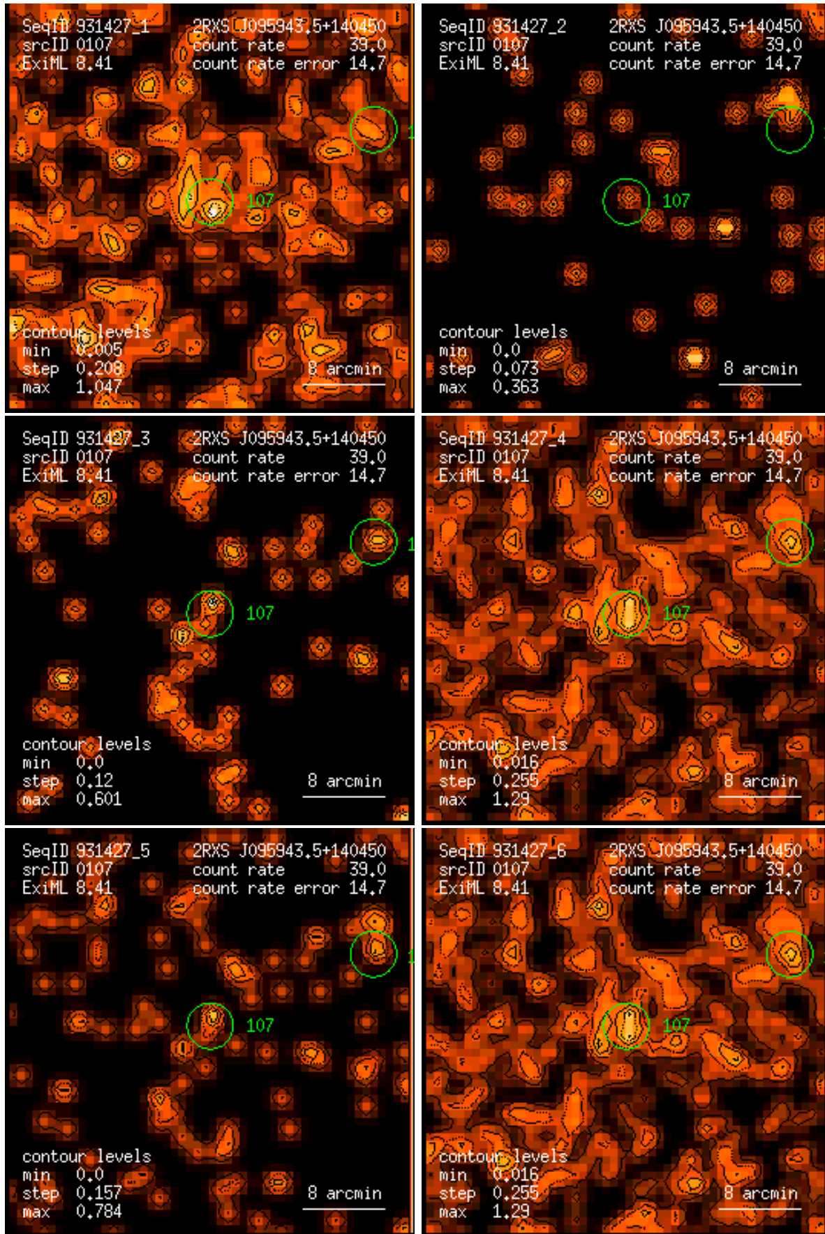
Figure 107: RASS 931427: detection 0107: band rate images, Gaussian filter: (1) PSPC channels 11 – 41, (2) 52 – 90, (3) 91 – 201, (4) 11 – 235, (5) 52 – 201, (6) 11 – 201. Broad band rates in counts/ks. Band rate contour levels in counts/ks/arcmin 2 .
