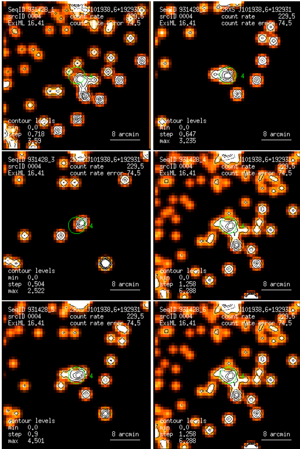
Figure 4: RASS 931428: detection 0004: band rate images, Gaussian filter: (1) PSPC channels 11 – 41, (2) 52 – 90, (3) 91 – 201, (4) 11 – 235, (5) 52 – 201, (6) 11 – 201. Broad band rates in counts/ks. Band rate contour levels in counts/ks/arcmin 2 .
