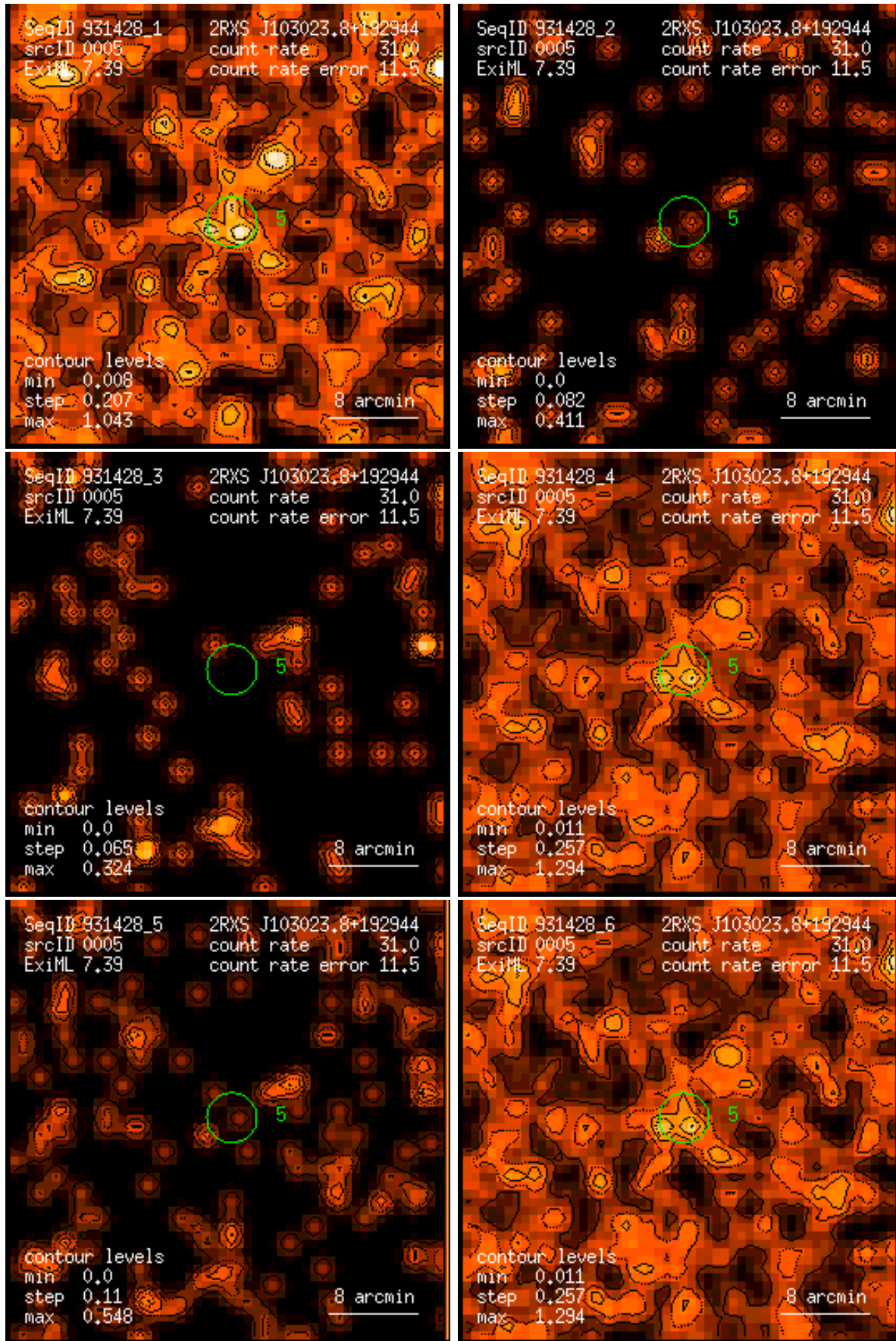
Figure 5: RASS 931428: detection 0005: band rate images, Gaussian filter: (1) PSPC channels 11 – 41, (2) 52 – 90, (3) 91 – 201, (4) 11 – 235, (5) 52 – 201, (6) 11 – 201. Broad band rates in counts/ks. Band rate contour levels in counts/ks/arcmin 2 .
