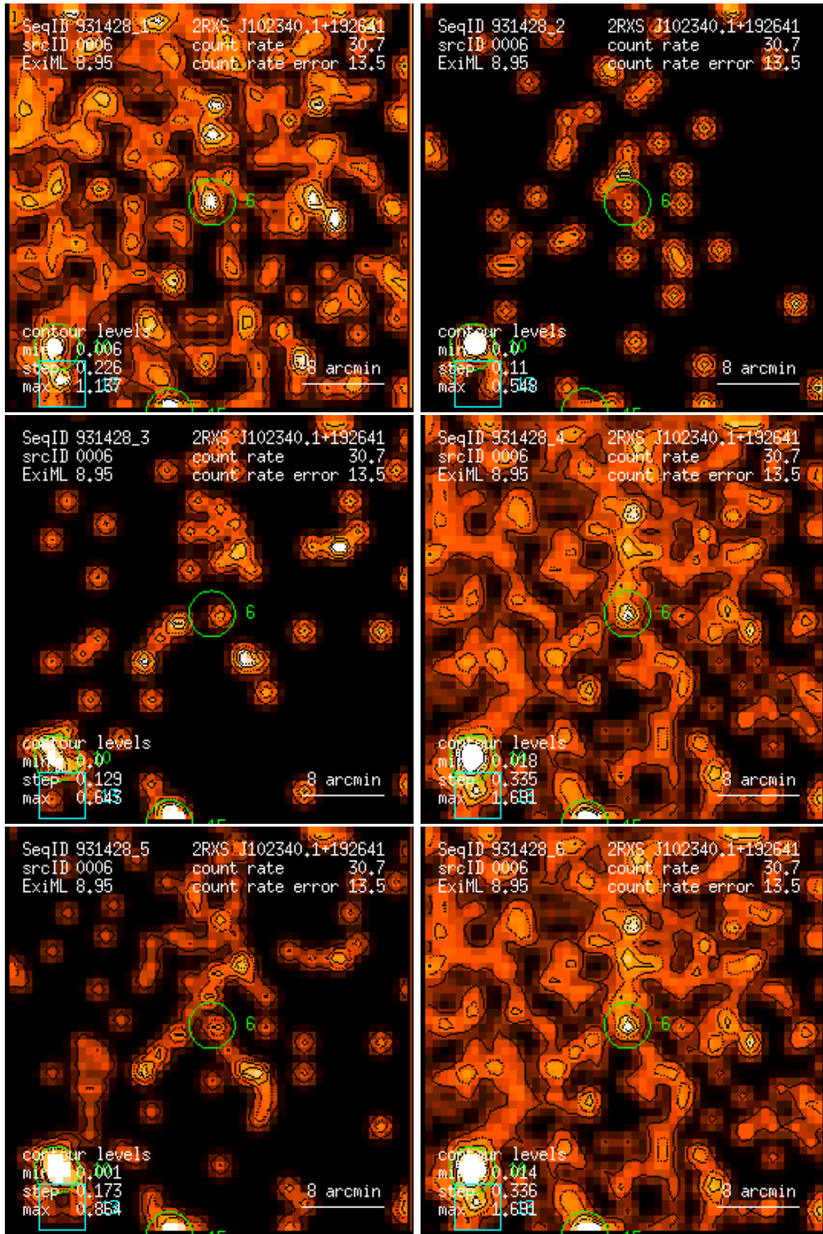
Figure 6: RASS 931428: detection 0006: band rate images, Gaussian filter: (1) PSPC channels 11 – 41, (2) 52 – 90, (3) 91 – 201, (4) 11 – 235, (5) 52 – 201, (6) 11 – 201. Broad band rates in counts/ks. Band rate contour levels in counts/ks/arcmin 2 .
