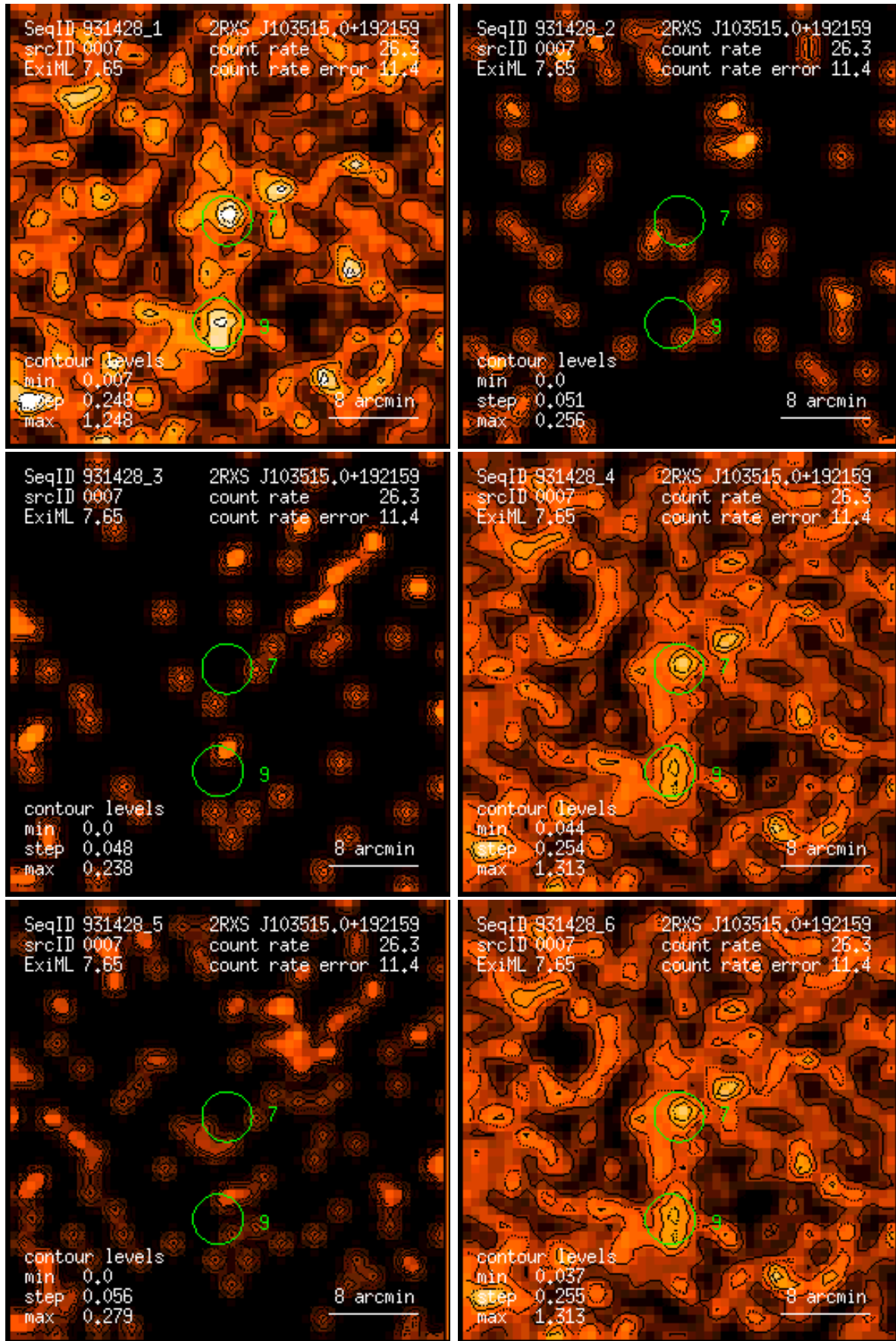
Figure 7: RASS 931428: detection 0007: band rate images, Gaussian filter: (1) PSPC channels 11 – 41, (2) 52 – 90, (3) 91 – 201, (4) 11 – 235, (5) 52 – 201, (6) 11 – 201. Broad band rates in counts/ks. Band rate contour levels in counts/ks/arcmin 2 .
