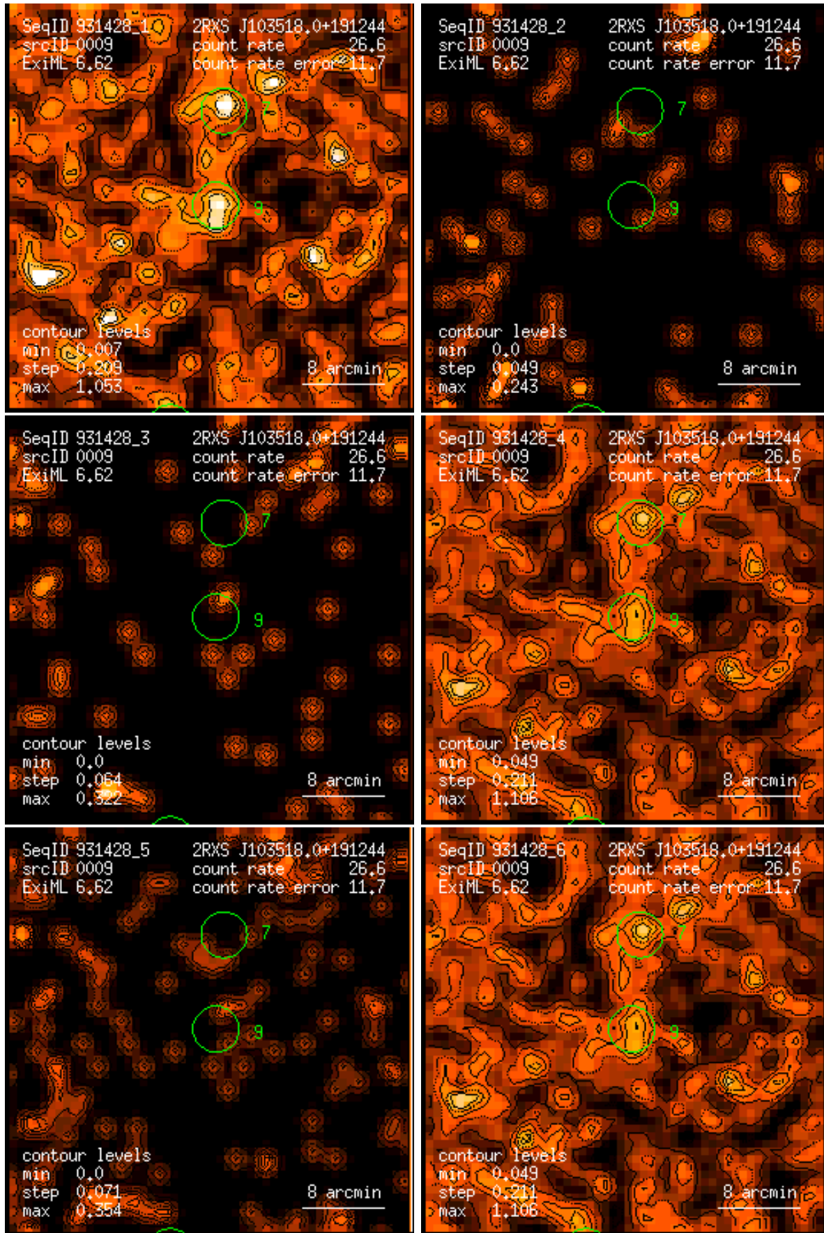
Figure 9: RASS 931428: detection 0009: band rate images, Gaussian filter: (1) PSPC channels 11 – 41, (2) 52 – 90, (3) 91 – 201, (4) 11 – 235, (5) 52 – 201, (6) 11 – 201. Broad band rates in counts/ks. Band rate contour levels in counts/ks/arcmin 2 .
