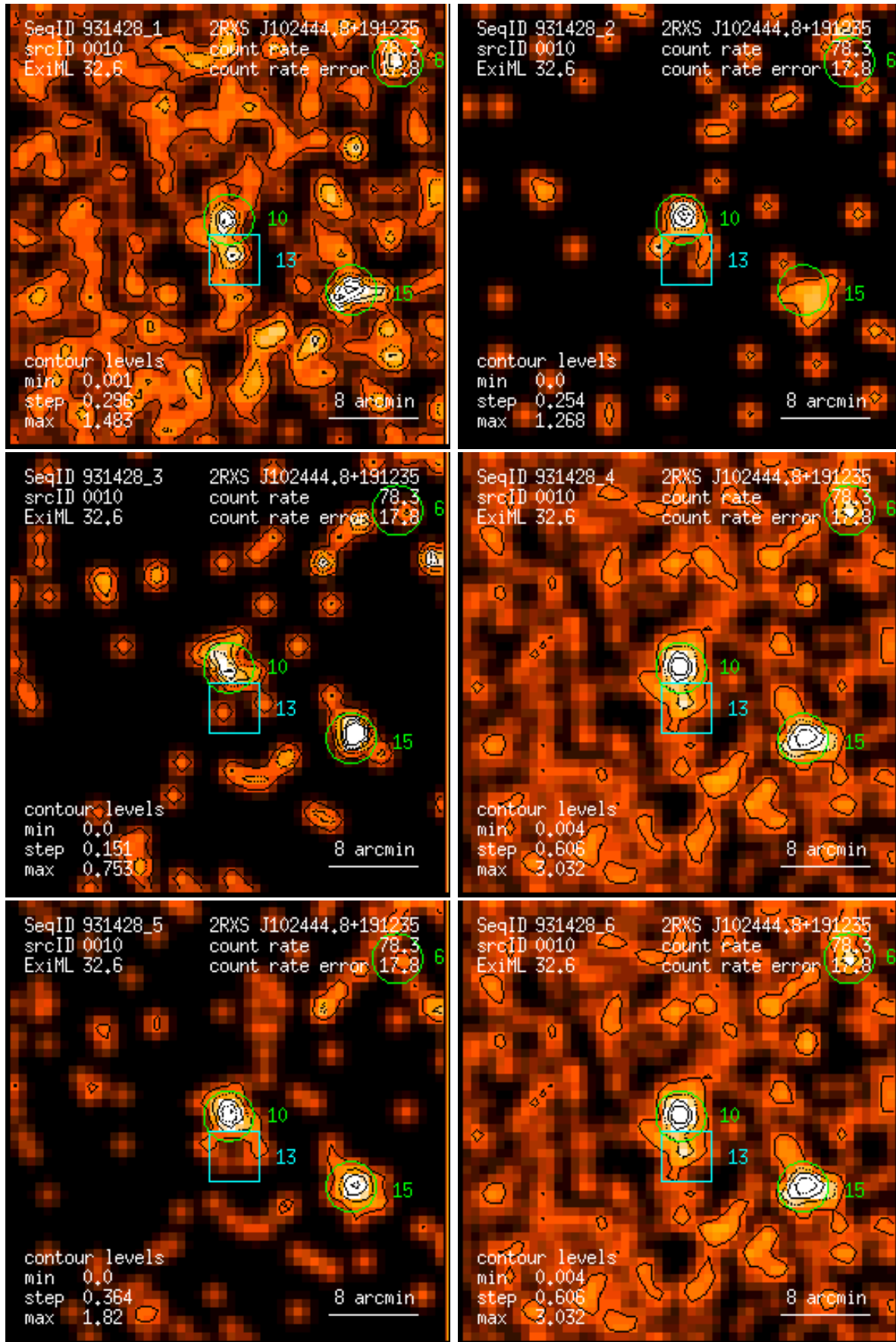
Figure 10: RASS 931428: detection 0010: band rate images, Gaussian filter: (1) PSPC channels 11 – 41, (2) 52 – 90, (3) 91 – 201, (4) 11 – 235, (5) 52 – 201, (6) 11 – 201. Broad band rates in counts/ks. Band rate contour levels in counts/ks/arcmin 2 .
