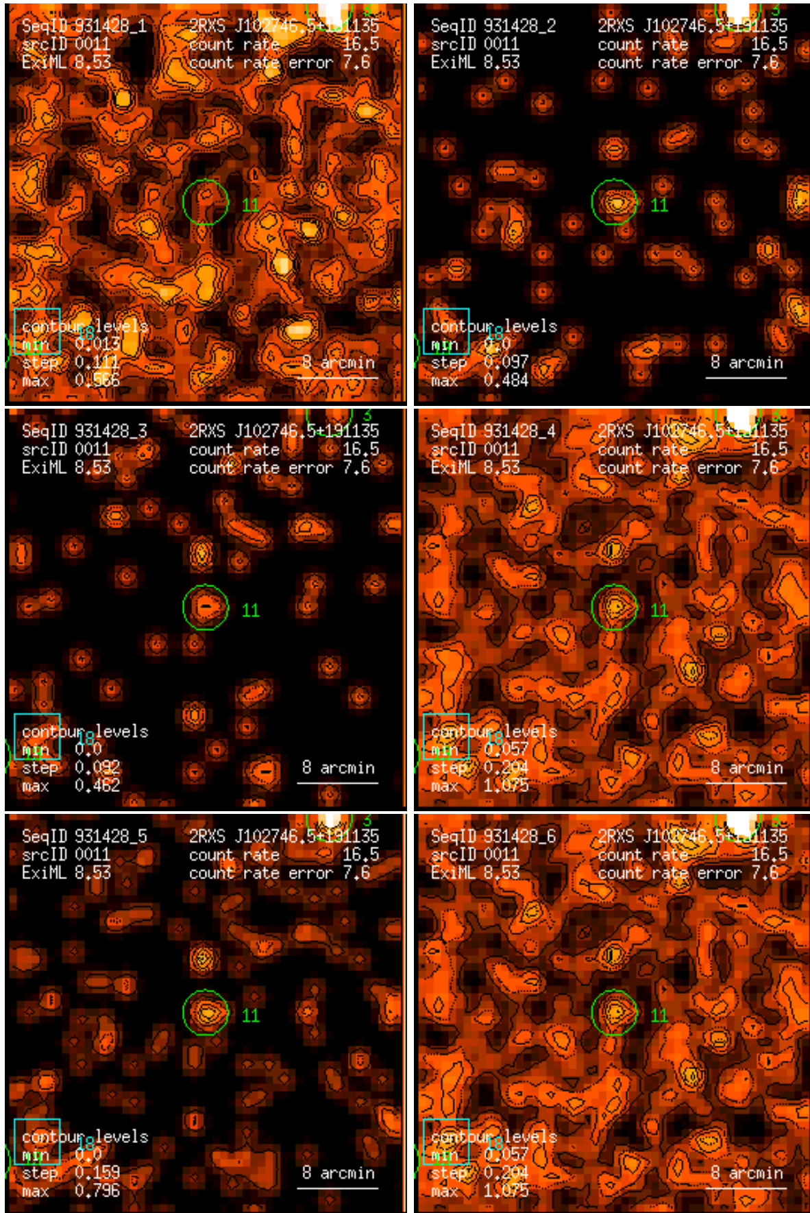
Figure 11: RASS 931428: detection 0011: band rate images, Gaussian filter: (1) PSPC channels 11 – 41, (2) 52 – 90, (3) 91 – 201, (4) 11 – 235, (5) 52 – 201, (6) 11 – 201. Broad band rates in counts/ks. Band rate contour levels in counts/ks/arcmin 2 .
