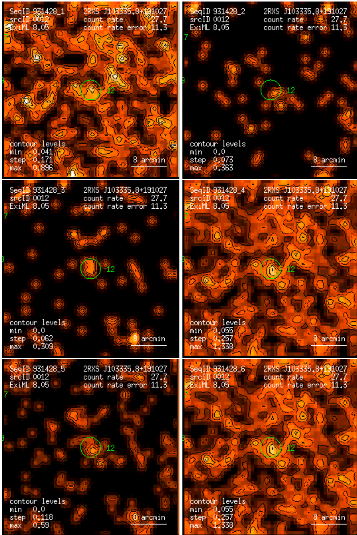
Figure 12: RASS 931428: detection 0012: band rate images, Gaussian filter: (1) PSPC channels 11 – 41, (2) 52 – 90, (3) 91 – 201, (4) 11 – 235, (5) 52 – 201, (6) 11 – 201. Broad band rates in counts/ks. Band rate contour levels in counts/ks/arcmin 2 .
