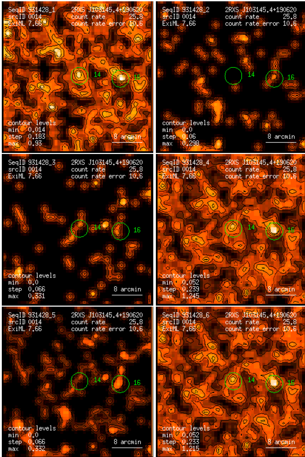
Figure 14: RASS 931428: detection 0014: band rate images, Gaussian filter: (1) PSPC channels 11 – 41, (2) 52 – 90, (3) 91 – 201, (4) 11 – 235, (5) 52 – 201, (6) 11 – 201. Broad band rates in counts/ks. Band rate contour levels in counts/ks/arcmin 2 .
