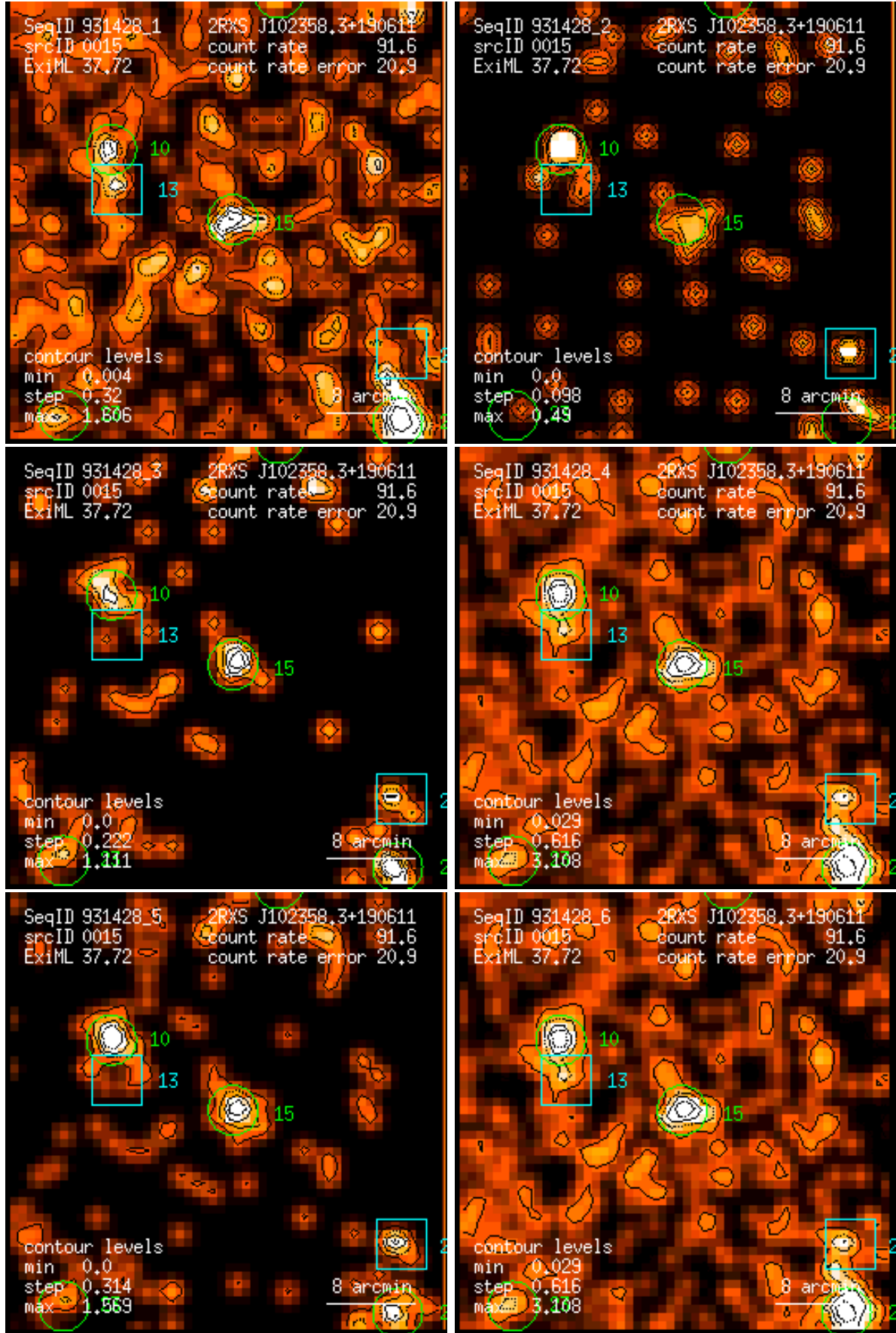
Figure 15: RASS 931428: detection 0015: band rate images, Gaussian filter: (1) PSPC channels 11 – 41, (2) 52 – 90, (3) 91 – 201, (4) 11 – 235, (5) 52 – 201, (6) 11 – 201. Broad band rates in counts/ks. Band rate contour levels in counts/ks/arcmin 2 .
