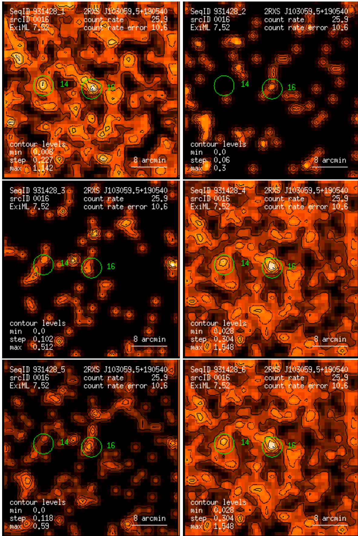
Figure 16: RASS 931428: detection 0016: band rate images, Gaussian filter: (1) PSPC channels 11 – 41, (2) 52 – 90, (3) 91 – 201, (4) 11 – 235, (5) 52 – 201, (6) 11 – 201. Broad band rates in counts/ks. Band rate contour levels in counts/ks/arcmin 2 .
